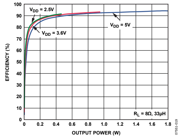
Figure 19. Efficiency vs. Output Power into 8\Omega + 33\mu H
