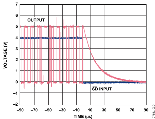
Figure 30. Turn-Off Response
