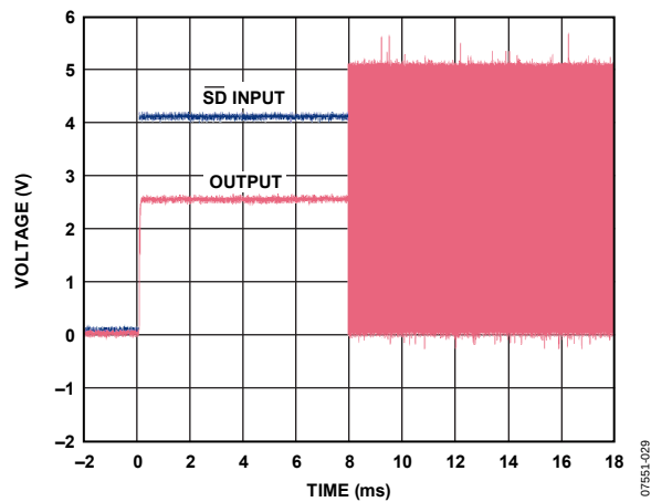
Figure 29. Turn-On Response
