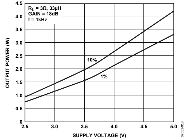
Figure 18. Maximum Output Power vs. Supply Voltage, R_L = 3\Omega + 33\mu H , Gain = 18 dB
