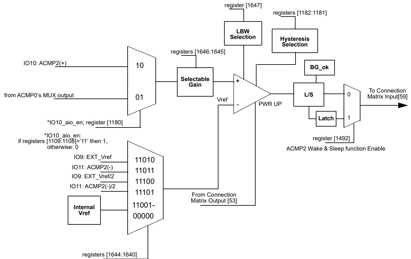
Figure 51: ACMP2 Block Diagram
