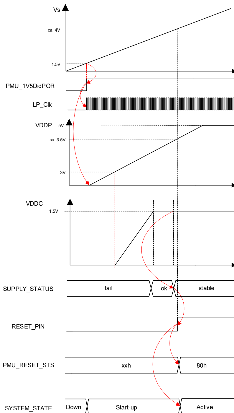
Figure 9 Power-on Reset Concept
