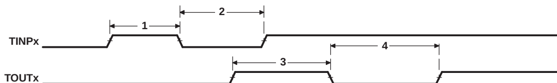
Figure 5-69. Timer Timing
