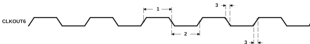
Figure 5-13. CLKOUT6 Timing
