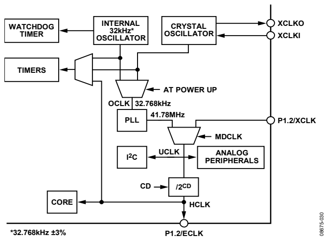
Figure 36. Clocking System
