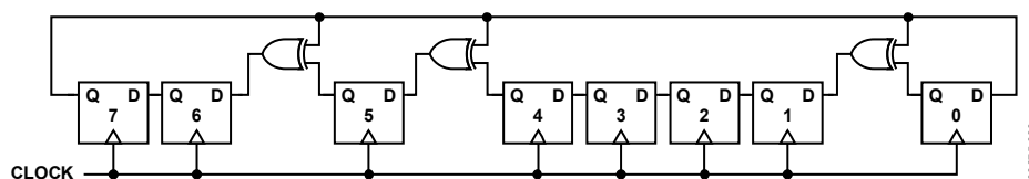
Figure 45. 8-Bit LFSR
