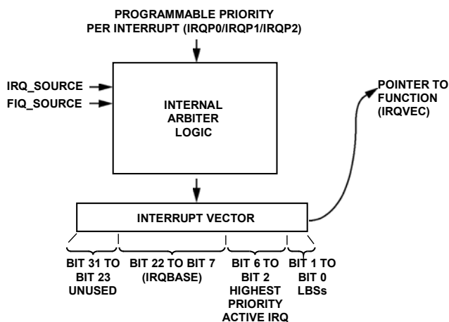
Figure 41. Interrupt Structure
