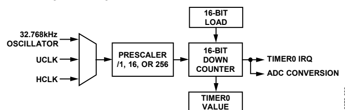
Figure 42. Timer0 Block Diagram
