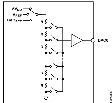
Figure 32. DAC Structure
