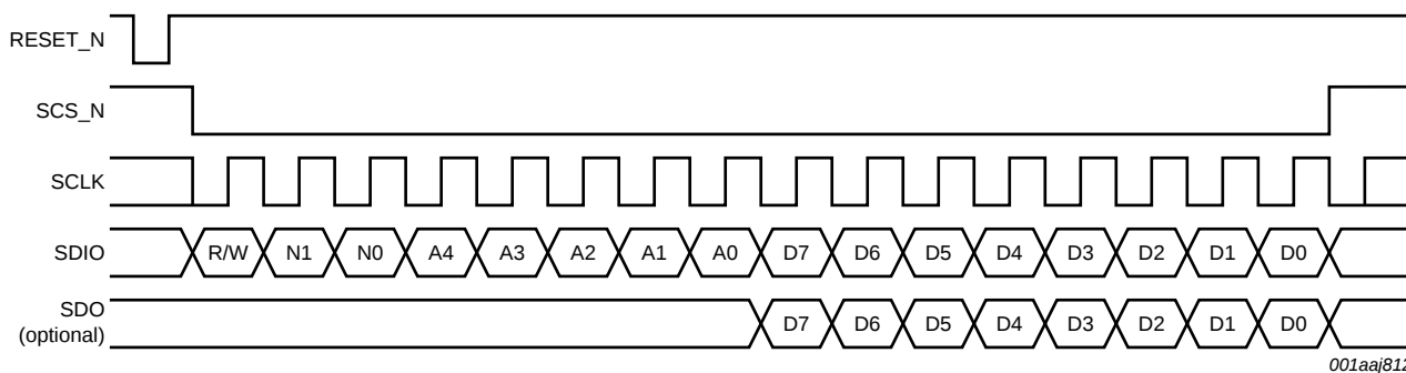
Fig 3. SPI protocol
