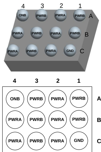
Figure 6. Bottom View
