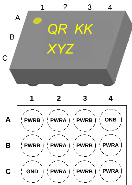
Figure 5. Top View
