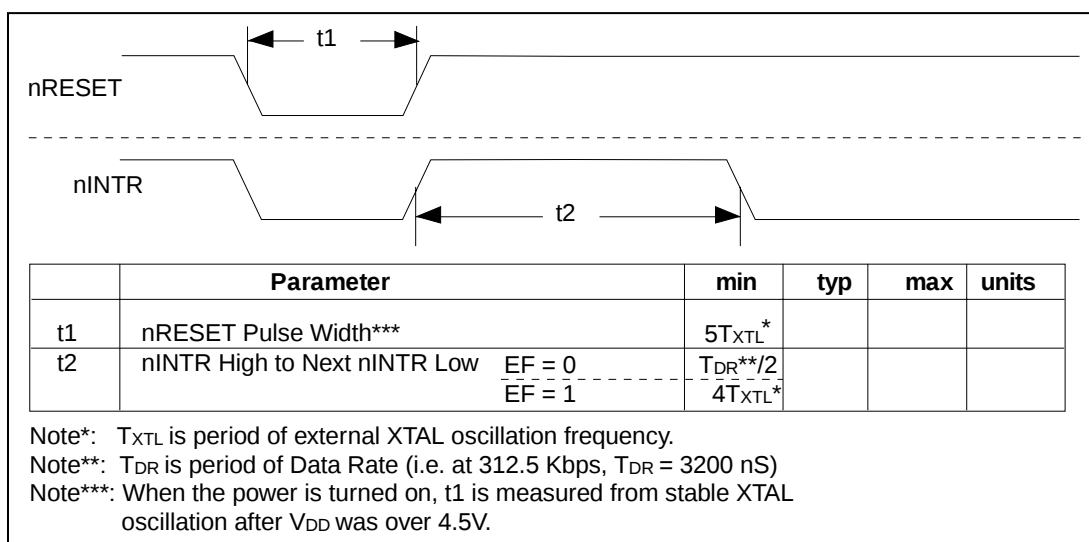
FIGURE 20 – RESET AND INTERRUPT TIMING
