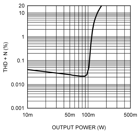
THD+N vs Output Power 3V, 8 \Omega , SE at 1kHz
