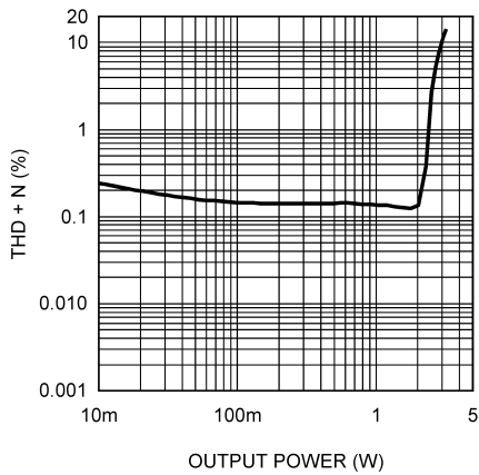
THD+N vs Output Power 5V, 3 \Omega , BTL at 1kHz
