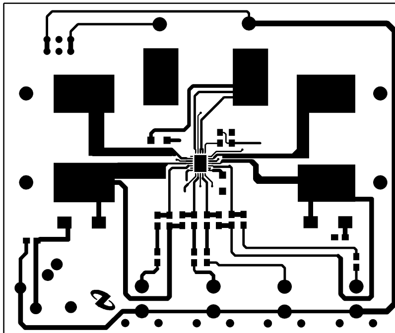
FIGURE 5. Top Layer
