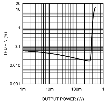
THD+N vs Output Power 5V, 32 \Omega , BTL at 1kHz
