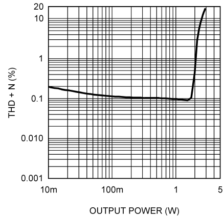
THD+N vs Output Power 5V, 4 \Omega , BTL at 1kHz
