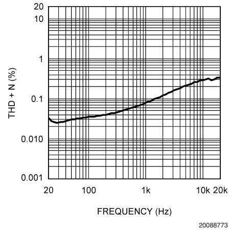
THD+N vs Frequency 3V, 32 \Omega , SE at 25mW
