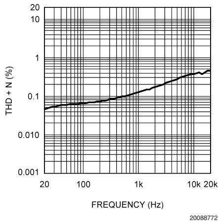
THD+N vs Frequency 3V, 4 \Omega , BTL at 250mW
