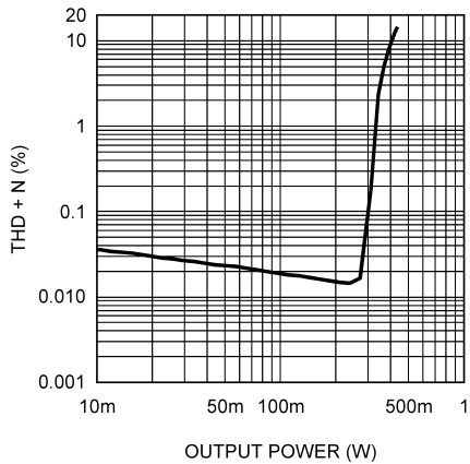
THD+N vs Output Power 5V, 8 \Omega , SE at 1kHz
