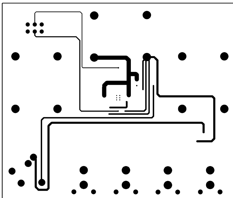
FIGURE 6. Bottom Layer
