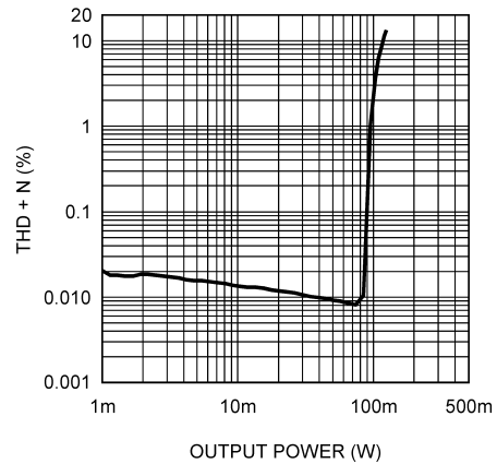
THD+N vs Output Power 5V, 32 \Omega , SE at 1kHz
