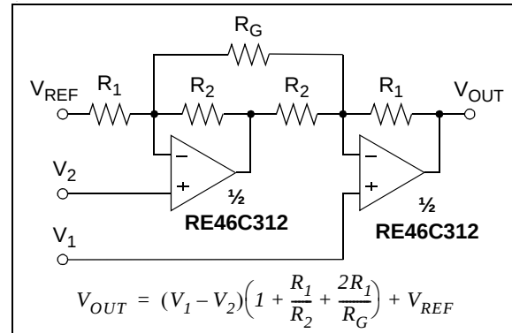
FIGURE 4-6: Two Op Amp Instrumentation Amplifier.
