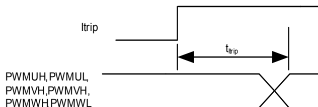
Figure 7 ITRIP timing
