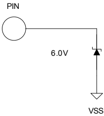
Figure 23 VDD1 and VDDCAP pin structure
