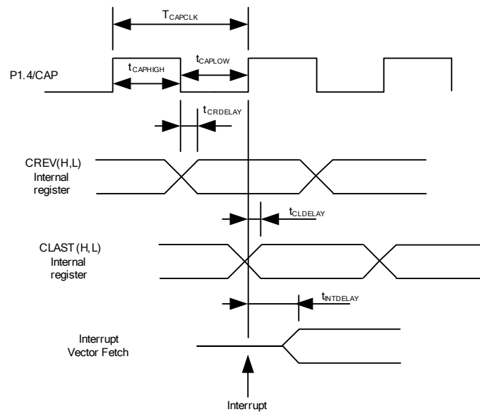
Figure 13 CAPTURE timing
