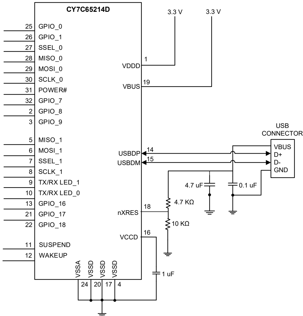
Figure 6. Self-Powered Configuration
