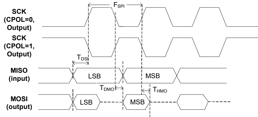
Figure 2. SPI Master Timing
