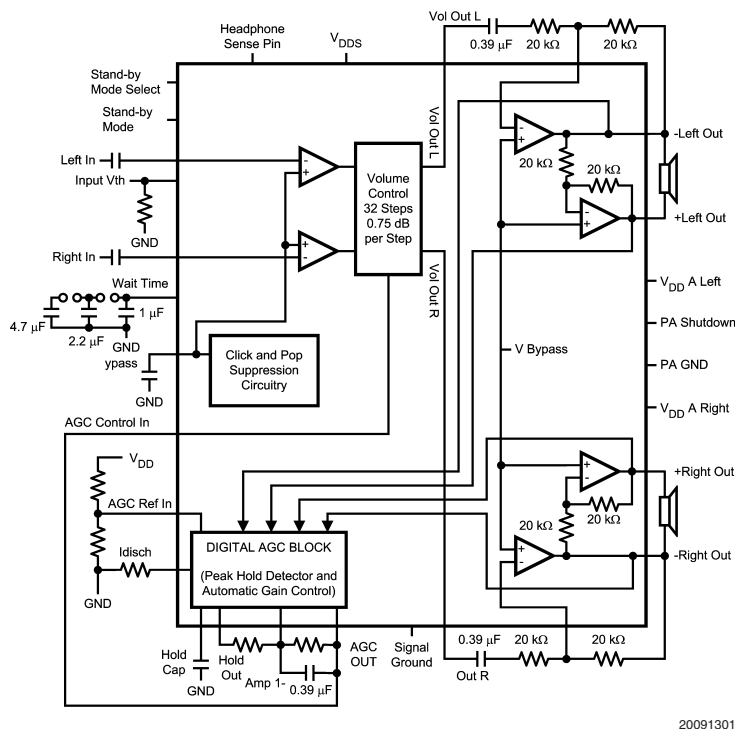
FIGURE 1. Typical Audio Amplifier Application Circuit
