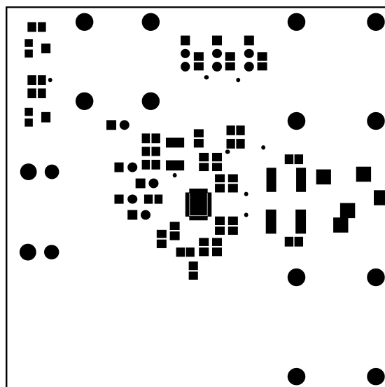
Top Solder
