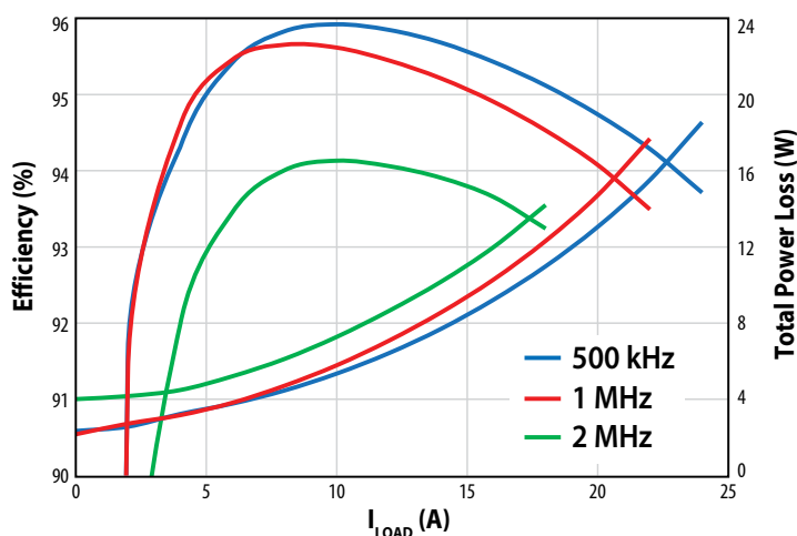
Figure 1: Performance Curves
