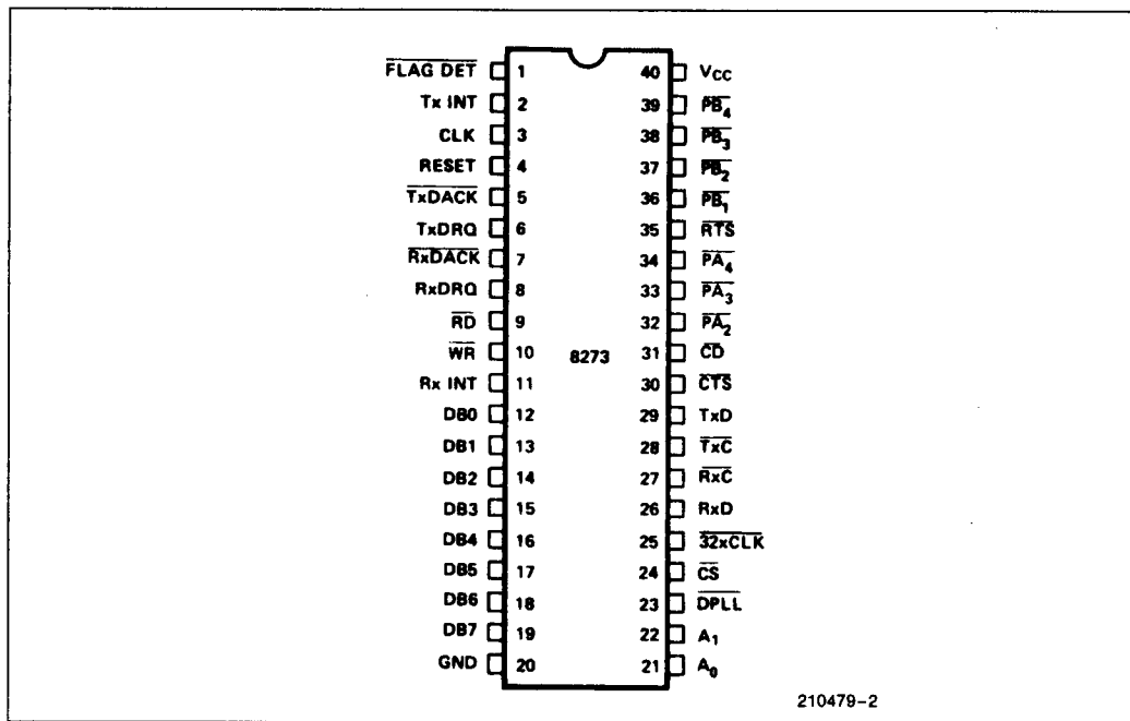
Figure 2. Configuration (PDIP)
