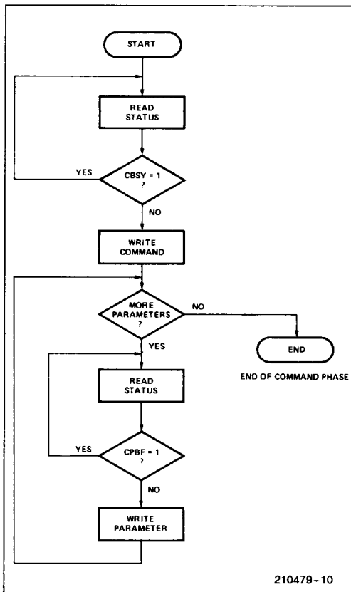
Figure 10. Command Phase Flowchart
