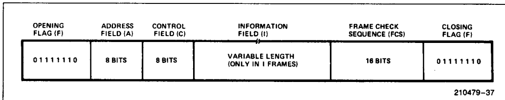
Figure 4. Frame Format
