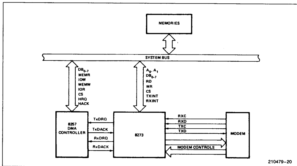
Figure 18. 8273 System Diagram
