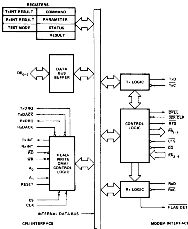
Figure 1. Block Diagram
