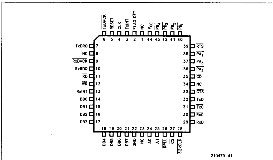
Figure 3. 8273 Pin Configuration (PLCC)
