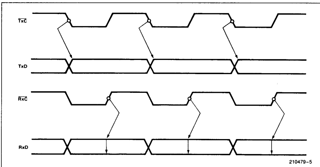
Figure 7. Transmit/Receive Timing
