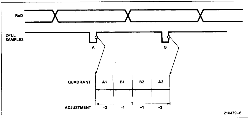
Figure 8. DPLL Sample Timing
