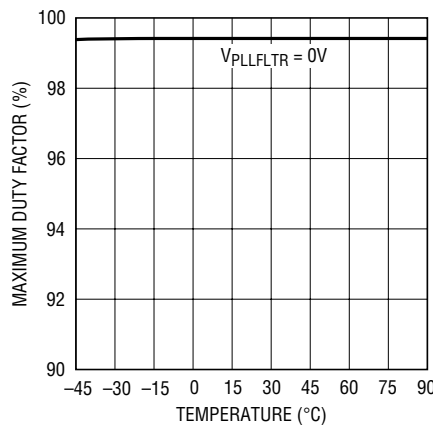
Maximum Duty Factors vs Temperature
