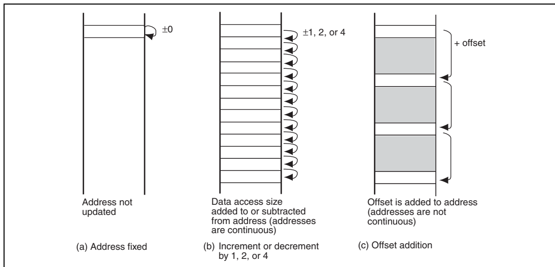
Figure 7.17 Address Update Method
