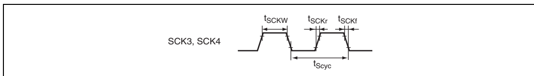
Figure 21.13 SCK Clock Input/Output Timing
