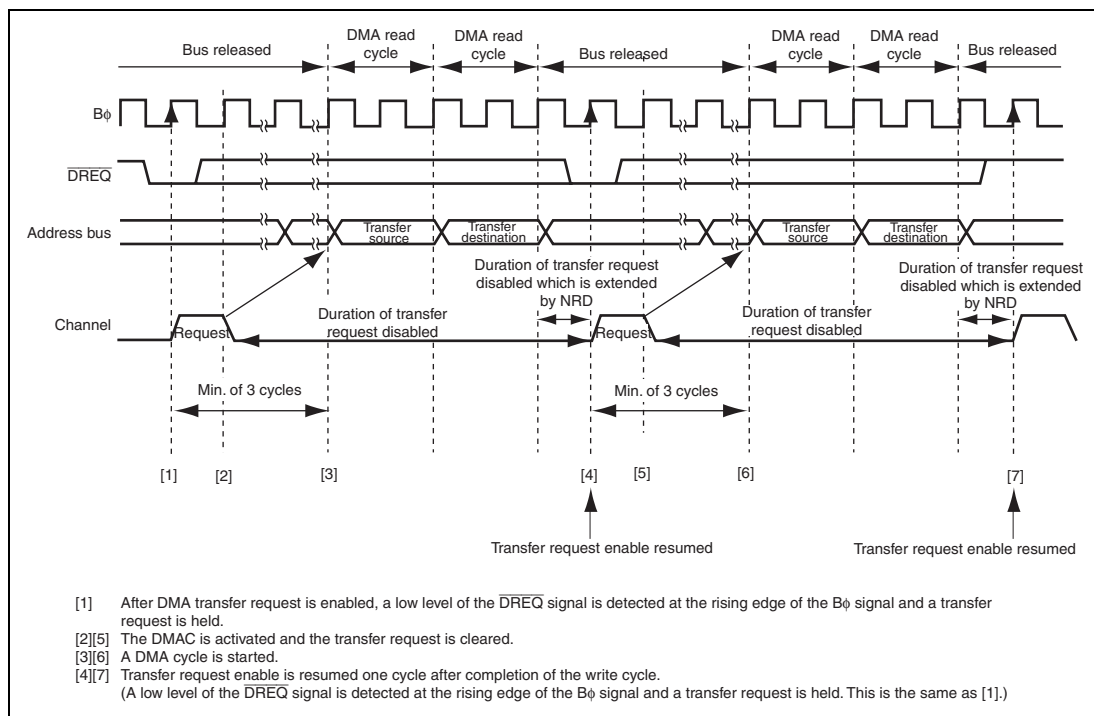
Figure 7.32 Example of Transfer in Normal Transfer Mode Activated by \overline{\text{DREQ}} Low Level with \text{NRD} = 1
