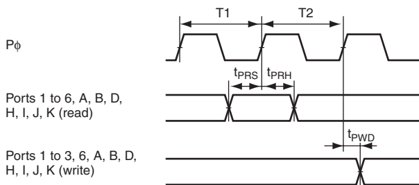
Figure 21.8 I/O Port Input/Output Timing
