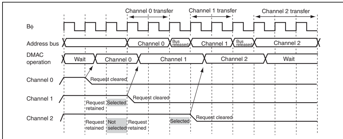
Figure 7.22 Example of Timing for Channel Priority
