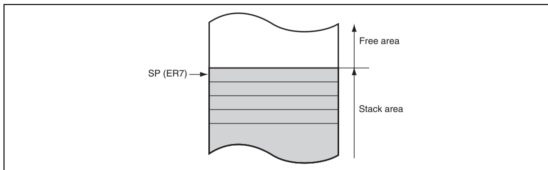
Figure 2.11 Stack
