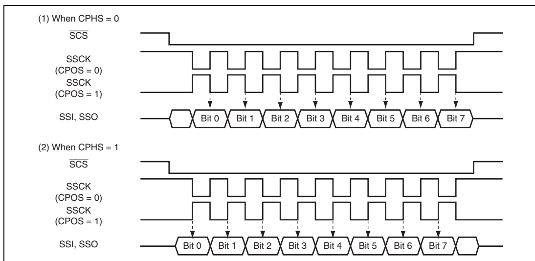
Figure 14.2 Relationship of Clock Phase, Polarity, and Data
