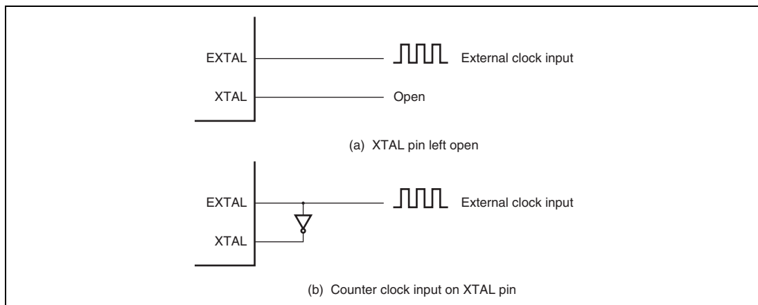
Figure 18.4 External Clock Input (Examples)
