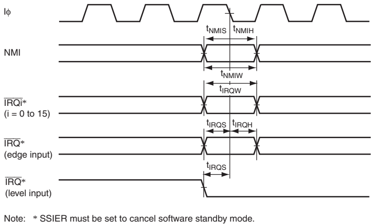
Figure 21.7 Interrupt Input Timing
