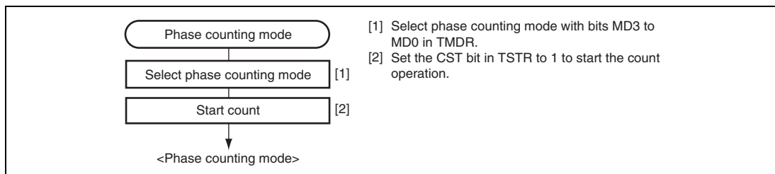
Figure 10.25 Example of Phase Counting Mode Setting Procedure
