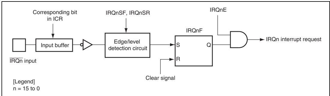
Figure 5.2 Block Diagram of Interrupts \overline{\text{IRQn}}
