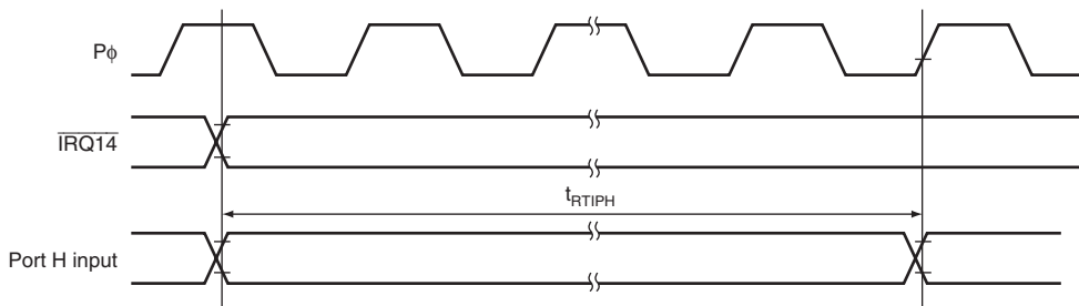
Figure 21.9 Data Input Timing for Realtime Input Port
