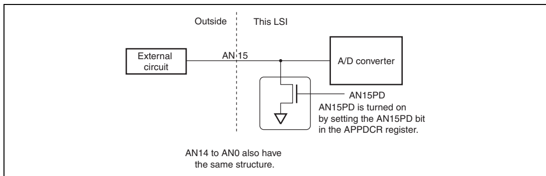
Figure 15.9 Diagram of Analog Port Pull-Down Function
