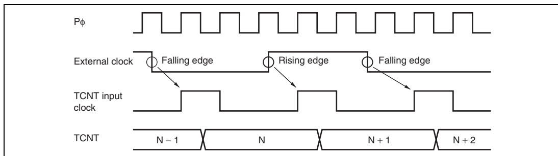
Figure 10.32 Count Timing in External Clock Operation
