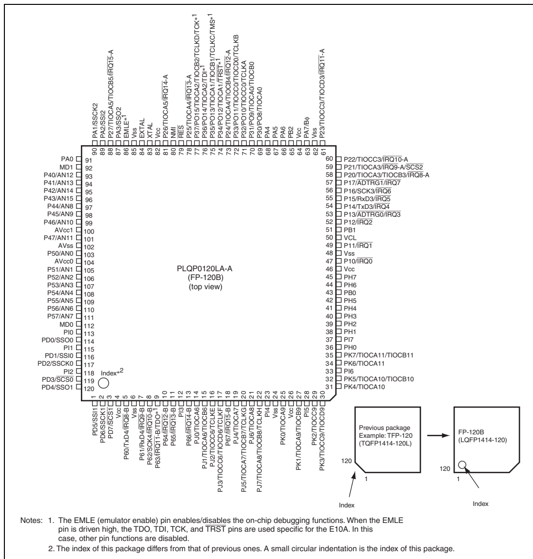
Figure 1.2 Pin Assignments of H8SX/1582
