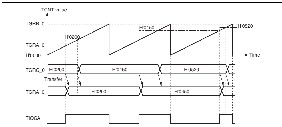
Figure 10.16 Example of Buffer Operation (1)
