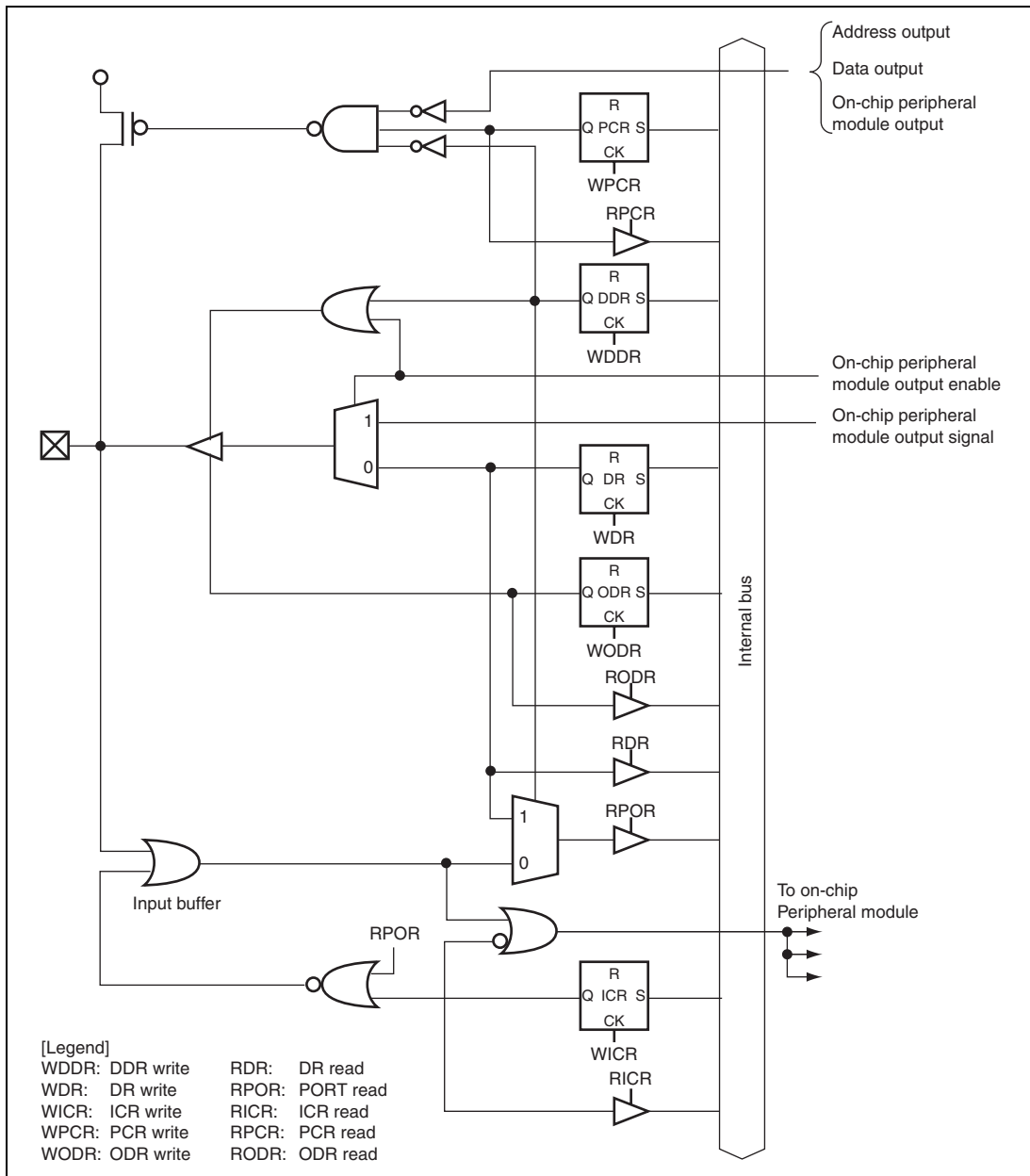
Figure 9.1 Port Block Diagram
