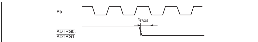
Figure 21.15 A/D Converter External Trigger Input Timing
