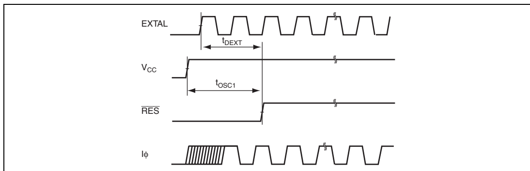
Figure 21.4 Oscillation Settling Timing
