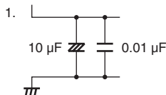
Figure 15.11 Example of Analog Input Protection Circuit
