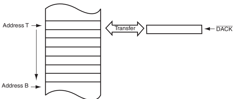
Figure 7.6 Operations in Single Address Mode
