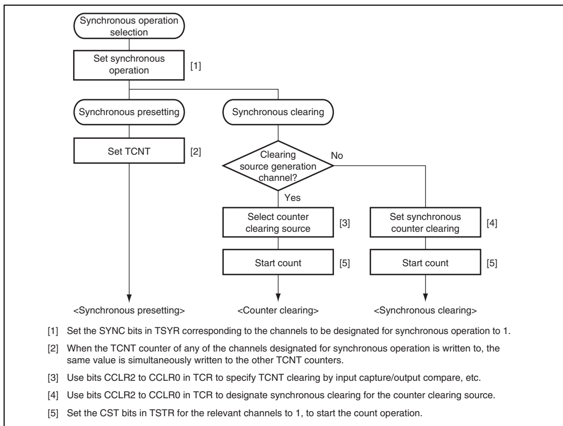
Figure 10.11 Example of Synchronous Operation Setting Procedure
