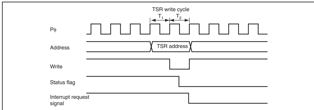
Figure 10.43 Timing for Status Flag Clearing by CPU
