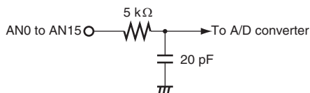
Figure 15.12 Analog Input Pin Equivalent Circuit
