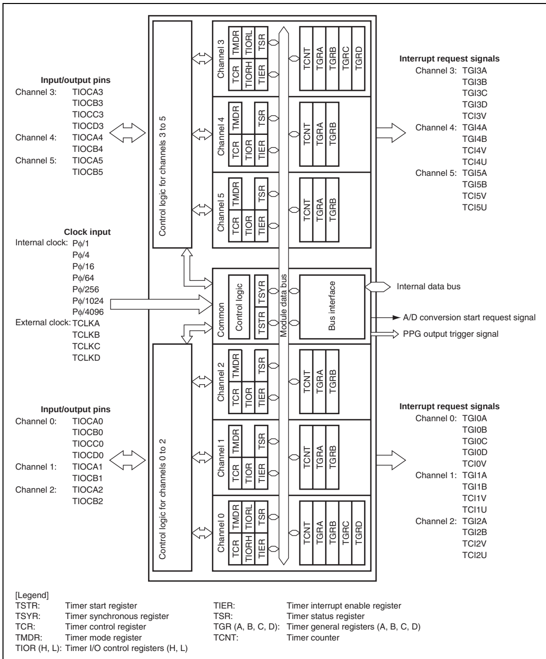
Figure 10.1 Block Diagram of TPU (Unit 0)
