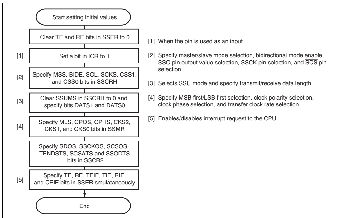
Figure 14.4 Example of Initial Settings in SSU Mode
