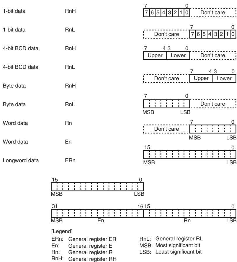
Figure 2.12 General Register Data Formats
