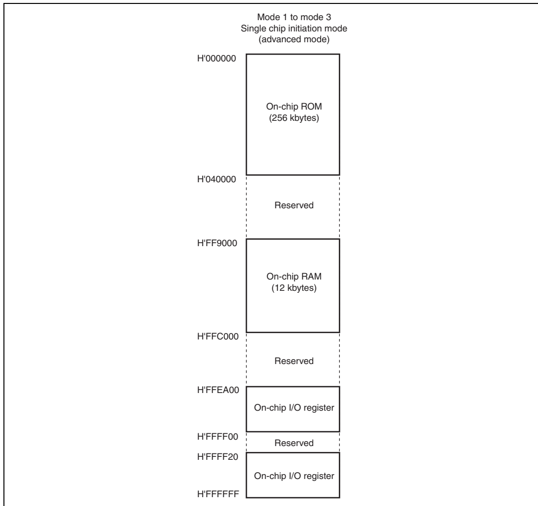
Figure 3.1 Address Map
