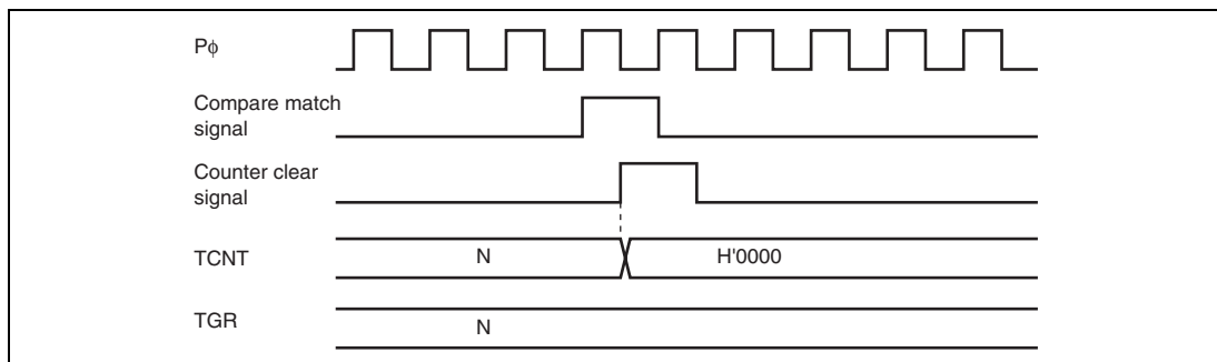
Figure 10.35 Counter Clear Timing (Compare Match)
