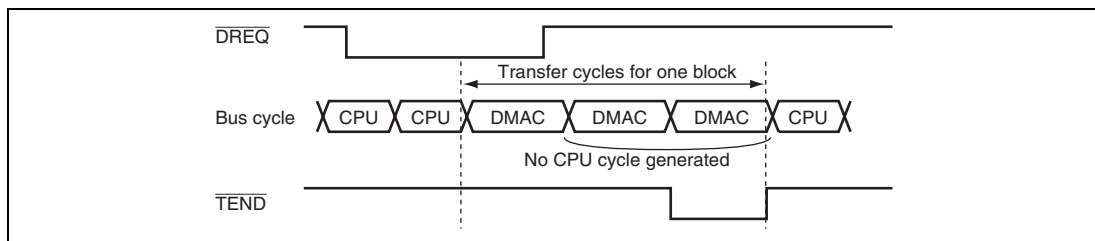
Figure 7.10 Operations in Block Transfer Mode
