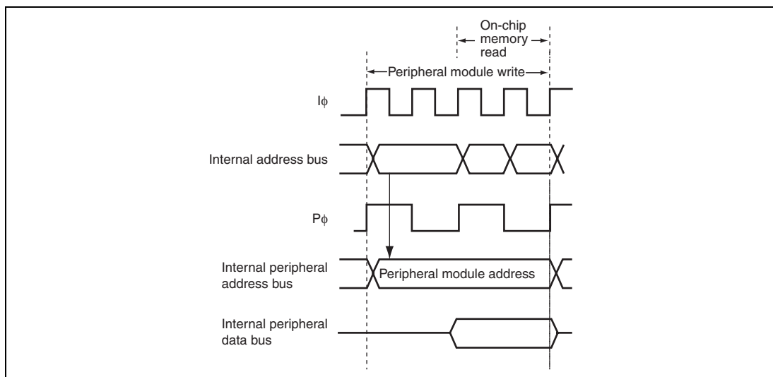
Figure 6.3 Example of Timing when Write Data Buffer Function is Used
