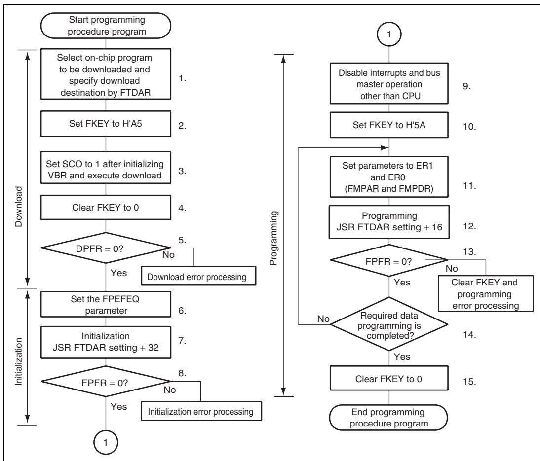
Figure 17.11 Programming Procedure in User Program Mode
