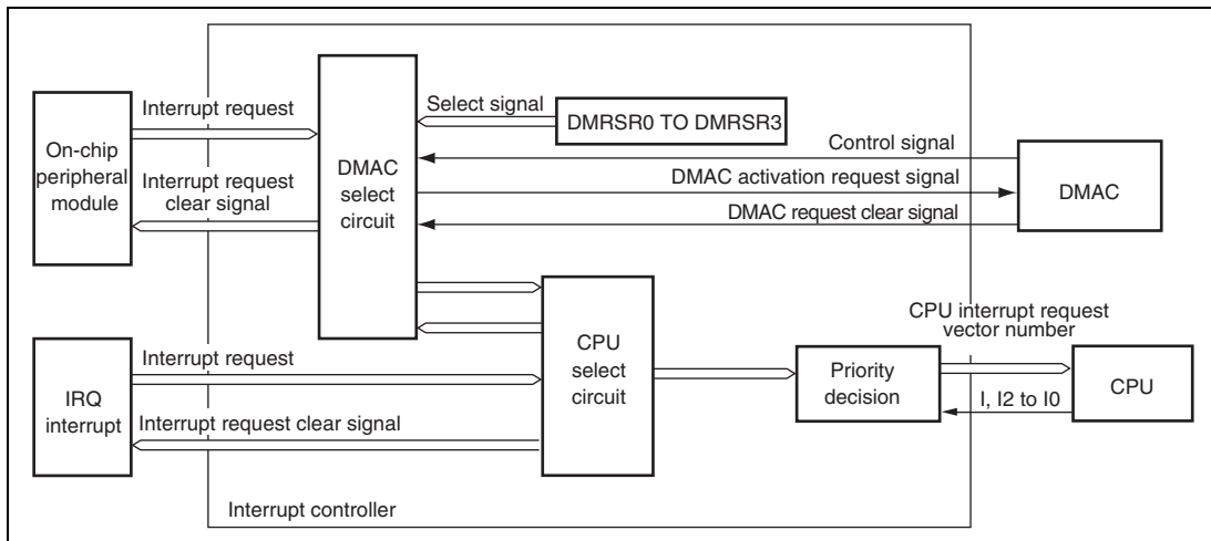
Figure 5.6 Block Diagram of DMAC and Interrupt Controller
