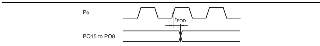
Figure 21.12 PPG Output Timing
