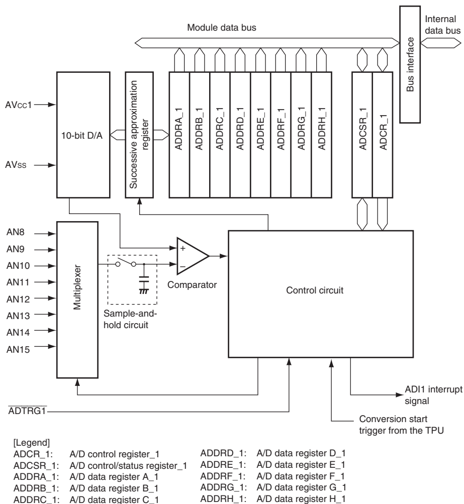
Figure 15.2 Block Diagram of A/D Converter (Unit 1/AD_1)
