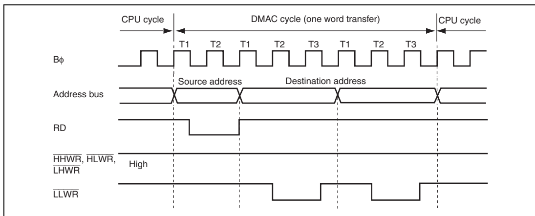
Figure 7.23 Example of Bus Timing of DMA Transfer
