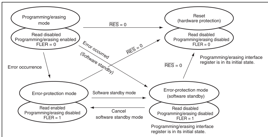
Figure 17.16 Transitions to Error Protection State
