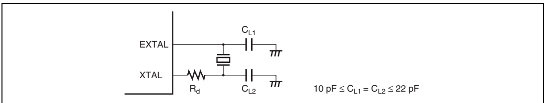
Figure 18.2 Connection of Crystal Resonator (Example)
