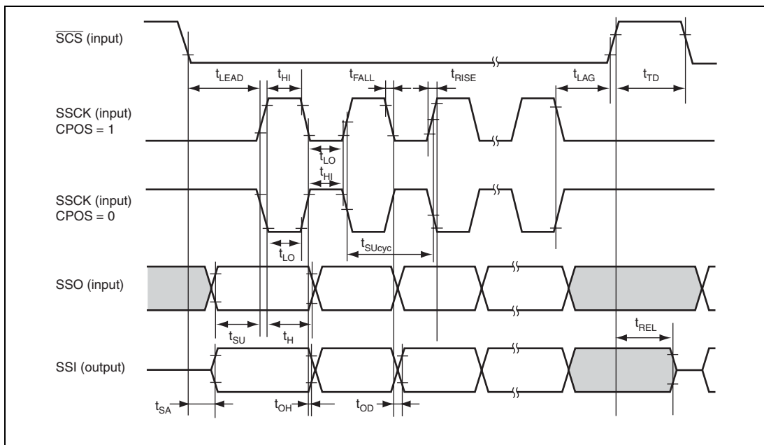
Figure 21.18 SSU Timing (Slave, CPHS = 1)
