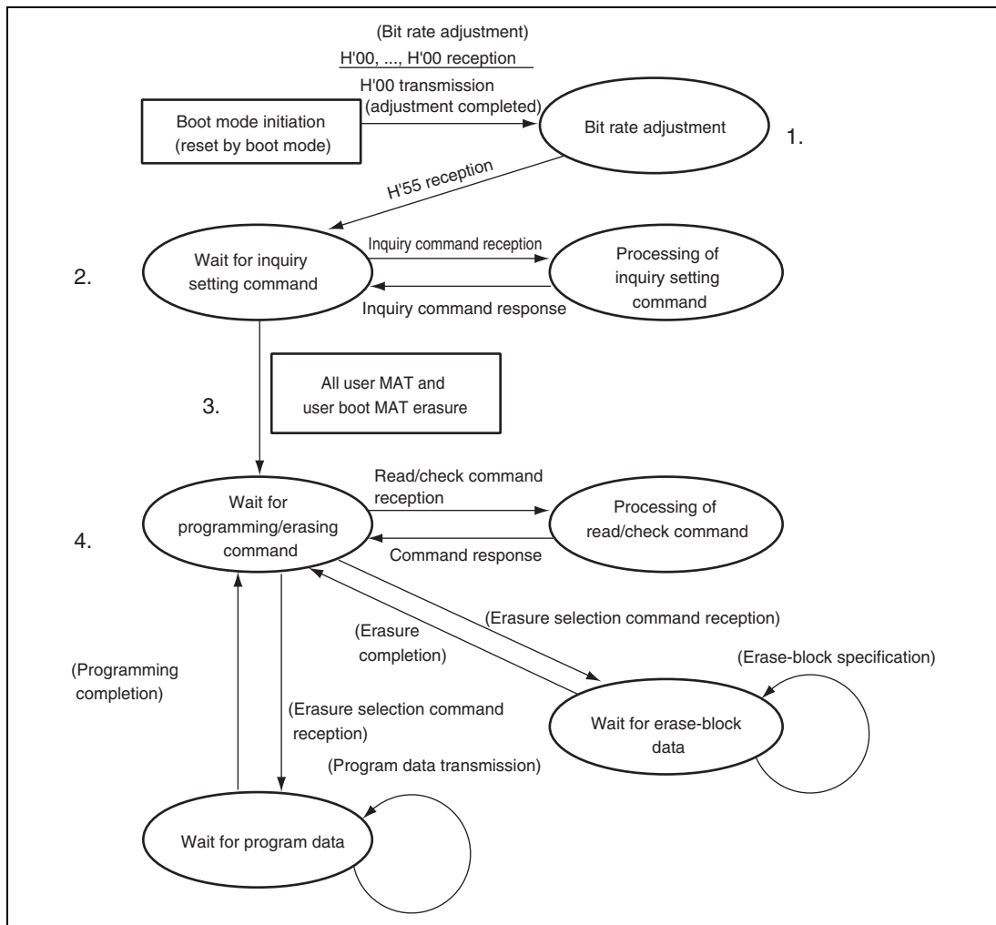
Figure 17.8 Boot Mode State Transition Diagram
