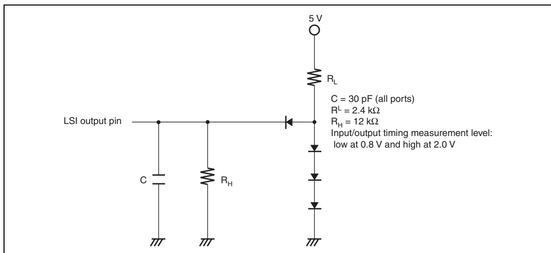
Figure 21.1 Output Load Circuit
