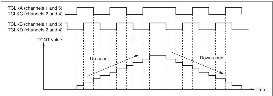
Figure 10.26 Example of Phase Counting Mode 1 Operation
