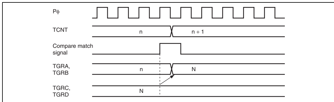
Figure 10.37 Buffer Operation Timing (Compare Match)
