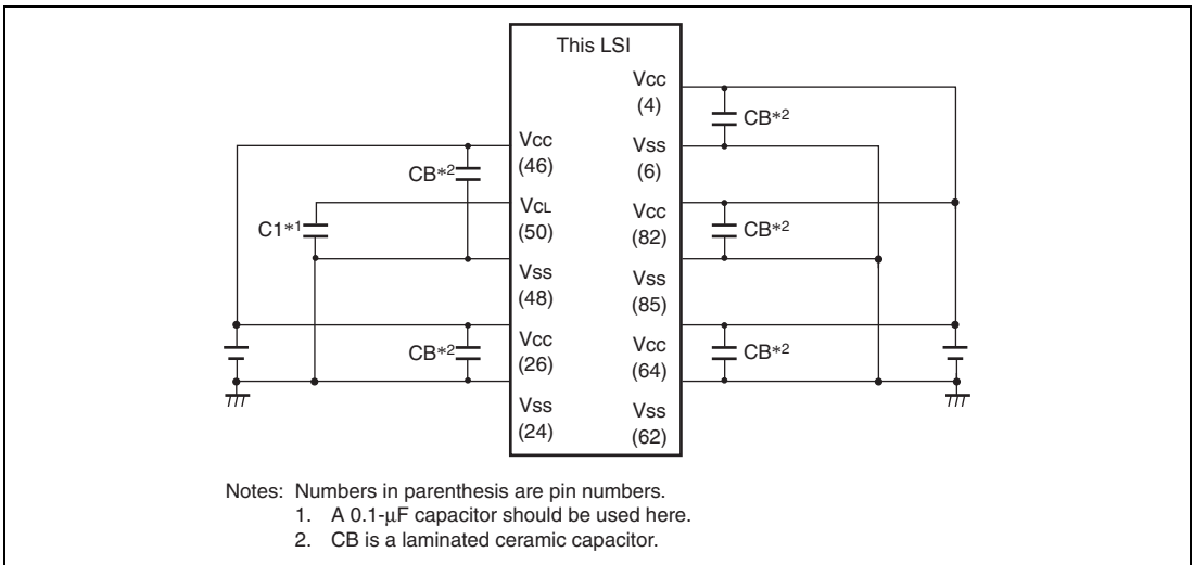
Figure 18.7 Connection Example of Bypass Capacitor
