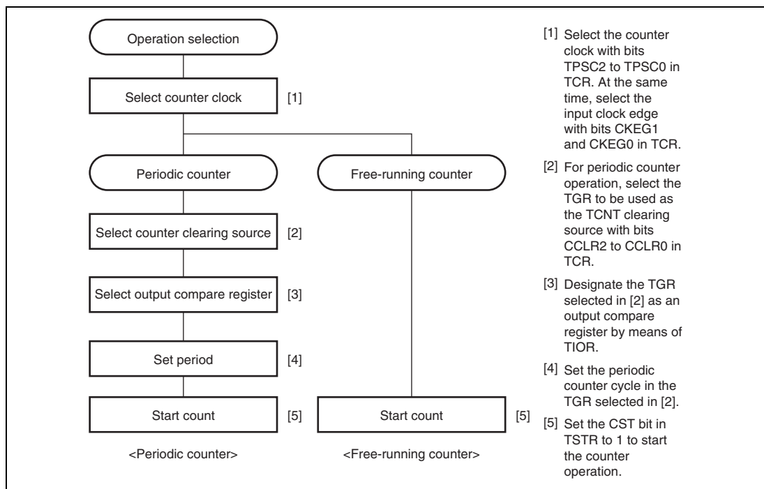
Figure 10.3 Example of Counter Operation Setting Procedure
