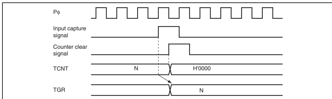
Figure 10.36 Counter Clear Timing (Input Capture)
