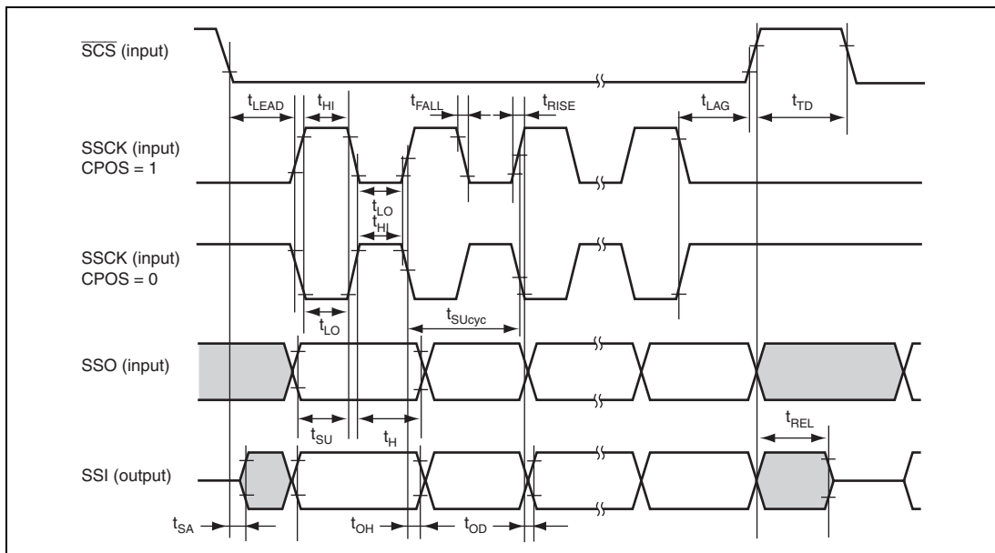
Figure 21.19 SSU Timing (Slave, CPHS = 0)
