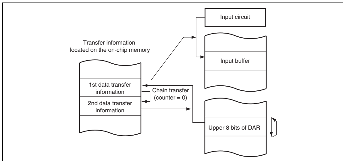
Figure 8.16 Chain Transfer when Counter = 0
