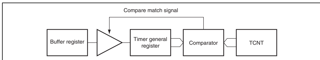
Figure 10.13 Compare Match Buffer Operation
