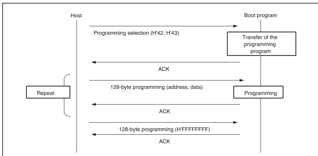
Figure 17.25 Programming Sequence
