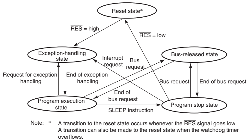
Figure 2.16 State Transitions
