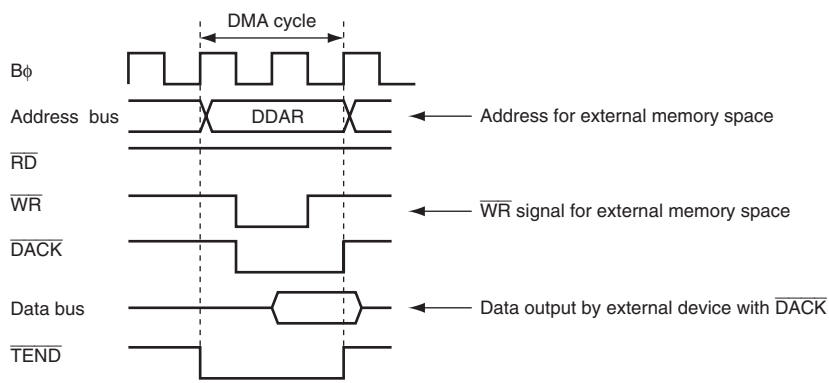
Figure 7.5 Example of Signal Timing in Single Address Mode
