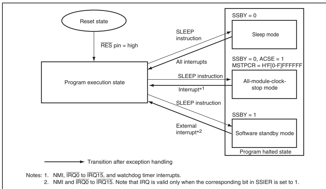
Figure 19.1 Mode Transitions
