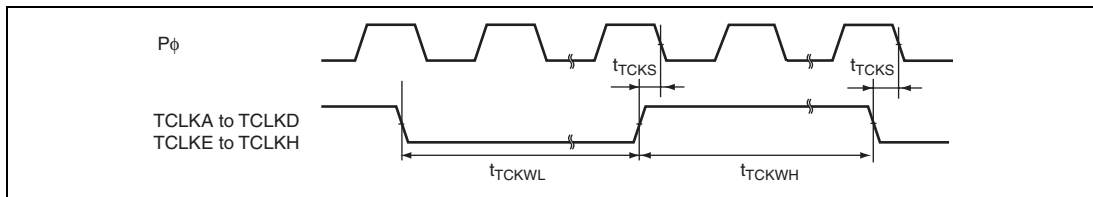
Figure 21.11 TPU Clock Input Timing
