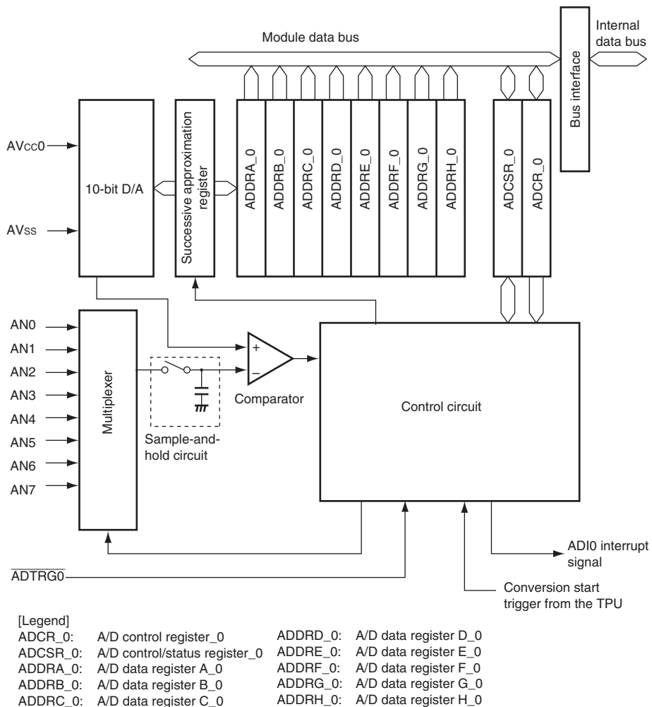
Figure 15.1 Block Diagram of A/D Converter (Unit 0/AD_0)
