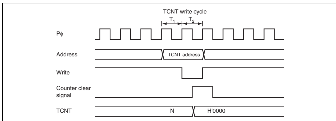
Figure 10.47 Conflict between TCNT Write and Clear Operations
