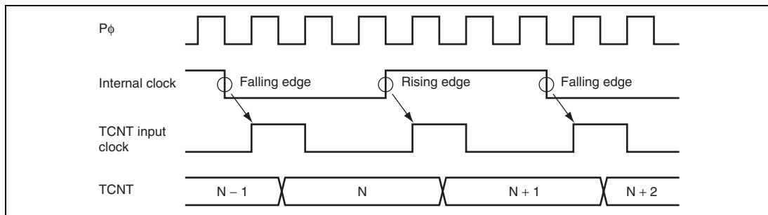
Figure 10.31 Count Timing in Internal Clock Operation
