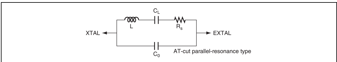
Figure 18.3 Crystal Resonator Equivalent Circuit
