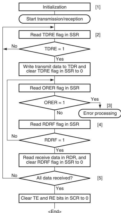
Figure 13.20 Sample Flowchart of Simultaneous Serial Transmission and Reception
