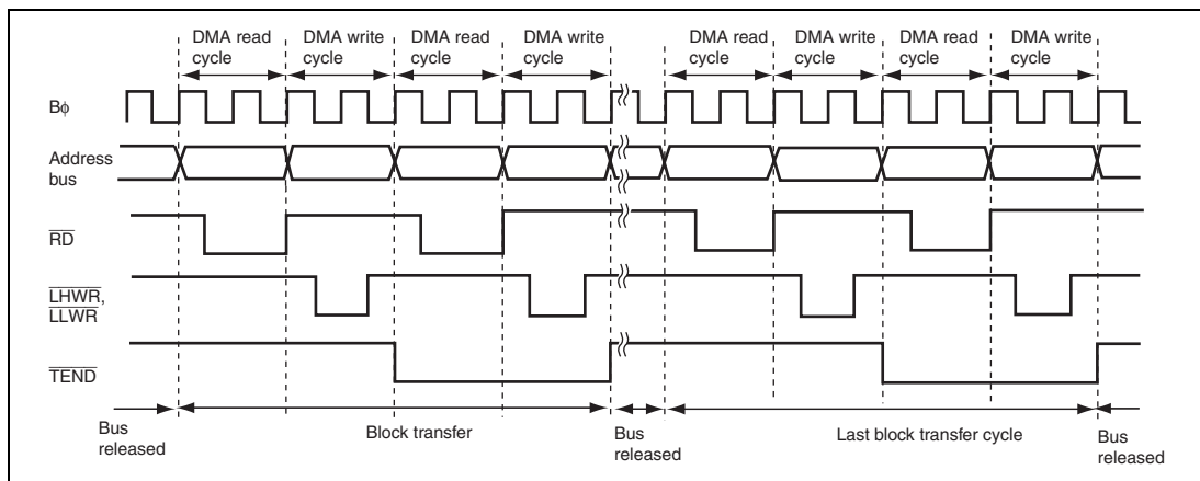
Figure 7.28 Example of Transfer in Block Transfer Mode
