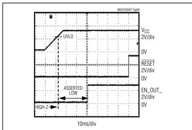
Figure 4. \overline{RESET} and EN\_OUT\_ During Power-Up, EN\_OUT\_ Is in Push-Pull Active-High Configuration
