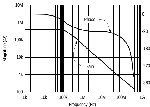
Transimpedance (ROL) vs Frequency
