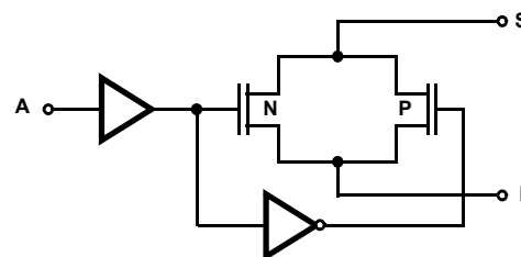
TYPICAL SWITCH
