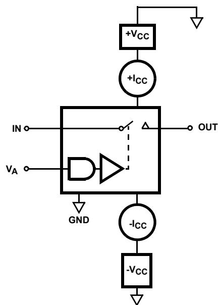
FIGURE 6. SUPPLY CURRENTS
