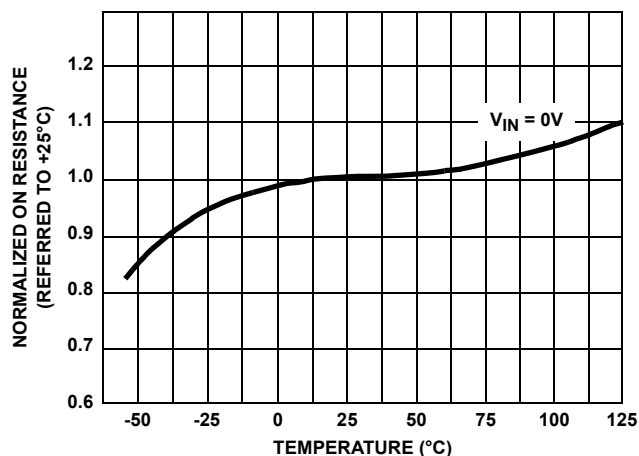
FIGURE 18. NORMALIZED ON RESISTANCE vs TEMPERATURE
