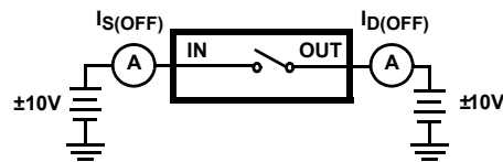
FIGURE 2. I_{S(OFF)}
