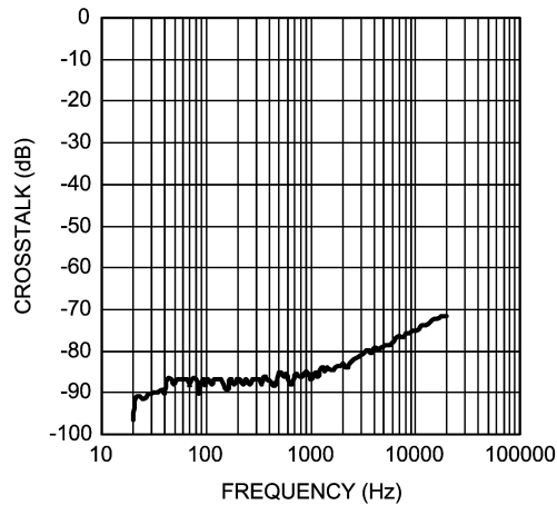
Crosstalk vs. Frequency V_{DD} = 3.6V , V_{RIPPLE} = 1\text{V}_{P-P} , R_L = 8\Omega
