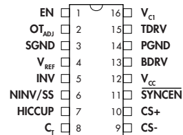
N PACKAGE (Top View)
