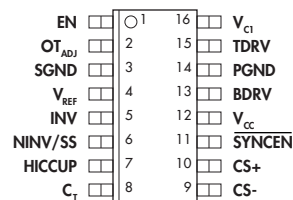
D PACKAGE (Top View)
