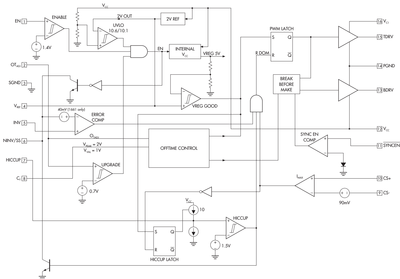
FIGURE 1 — Block Diagram
