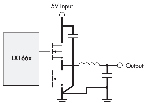
FIGURE 10 — Power Traces
