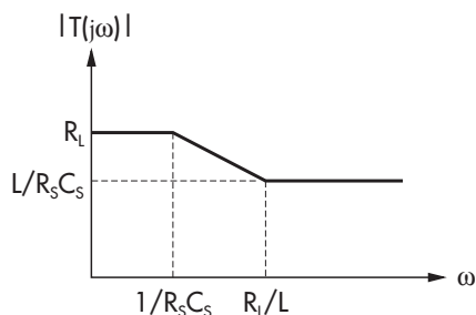
FIGURE 9 — Sensor Gain
