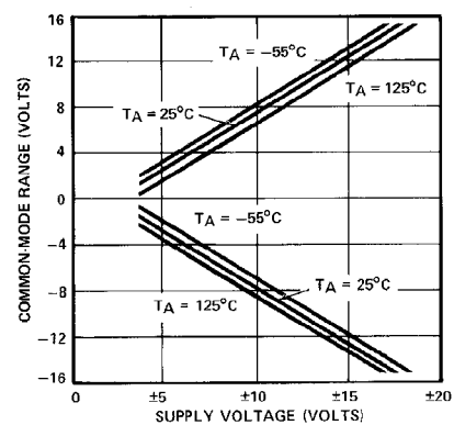
COMMON-MODE INPUT RANGE vs SUPPLY VOLTAGE
