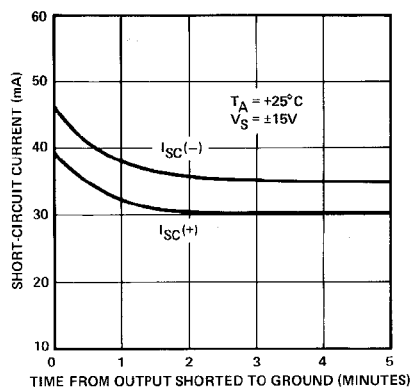
SHORT-CIRCUIT CURRENT vs TIME
