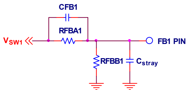
Figure 22. Addition of CFB1 to cancel stray capacitance
