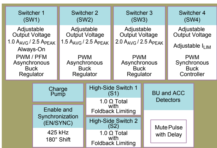
Figure 1. A8600 major features
