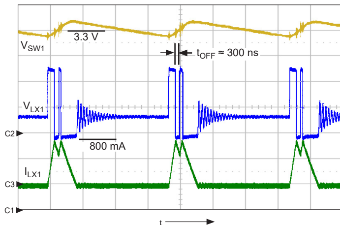
Figure 12. SW1 PFM operation at V_{IN1} = 12 V, V_{SW1} = 3.3 V, V_{SW1} = 120 mA load, LX1 turns on twice every 18 \mu s to regulate V_{SW1} ; shows V_{SW1} (ch1, 100 mV/div.), V_{LX1} (ch2, 5 V/div.), I_{LX1} (ch3, 500 mA/div.), t = 5 \mu s/div.
