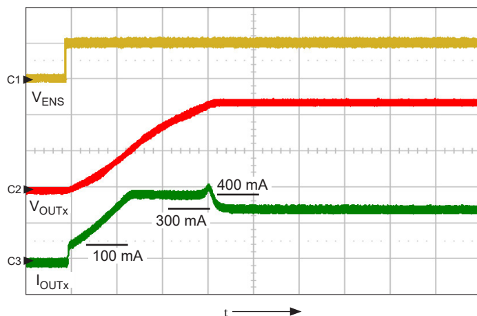
Figure 16. S1/S2 OUTx turning on with a load of 40 Ω and 22 μF; shows V ENS (ch1, 5 V/div.), V OUTx (ch2, 5 V/div.), I OUTx (ch3, 200 mA/div.), t = 500 μs/div.
