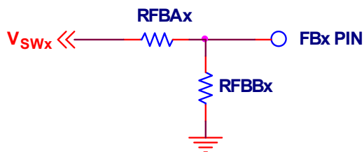
Figure 21. Connecting the feedback divider
