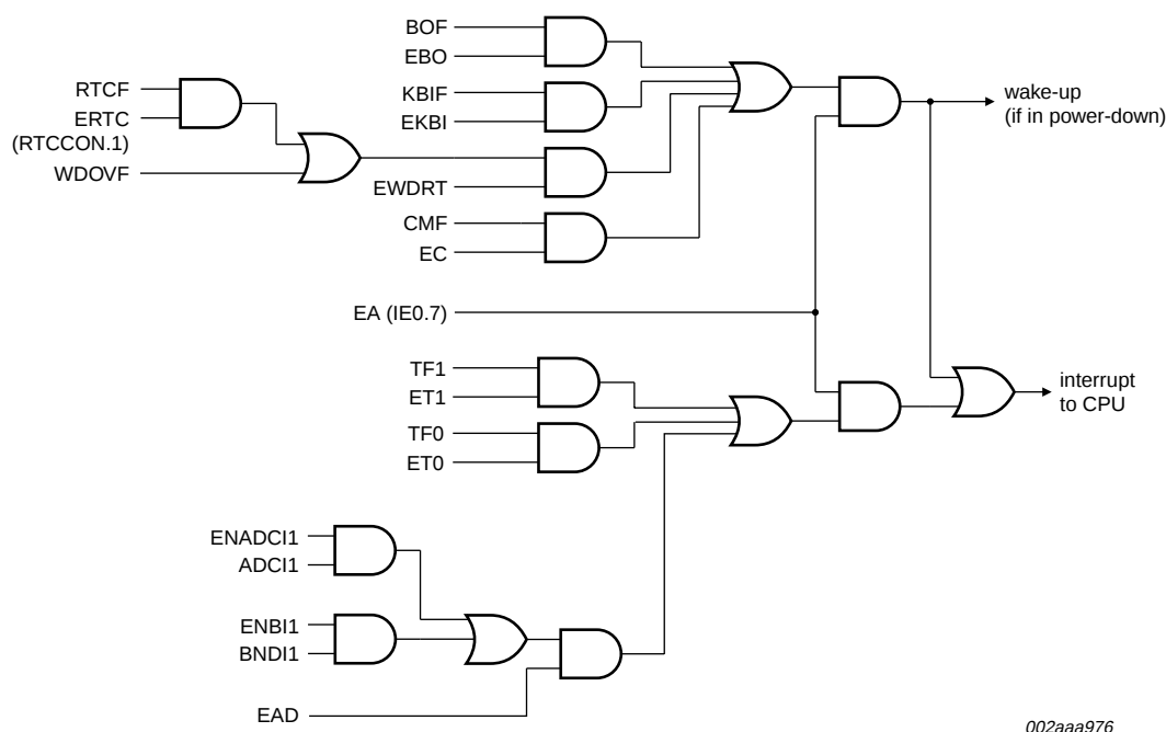
Fig 13. Interrupt sources, interrupt enables, and power-down wake-up sources (P89LPC9102)
