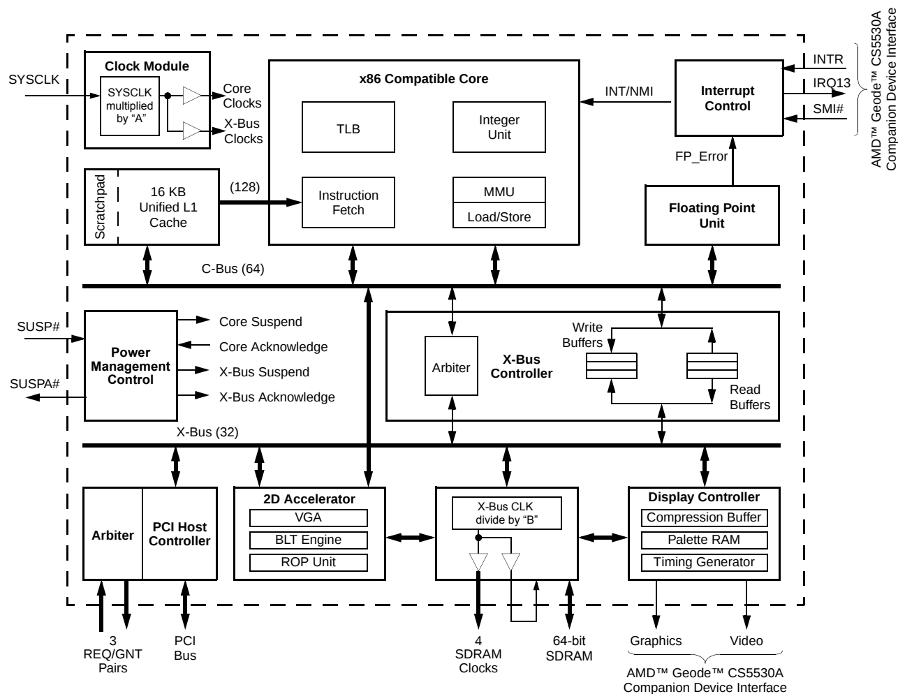
Figure 1-1. Block Diagram
