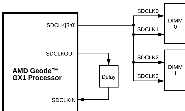
Figure 5-9. SDCLKIN Clocking
