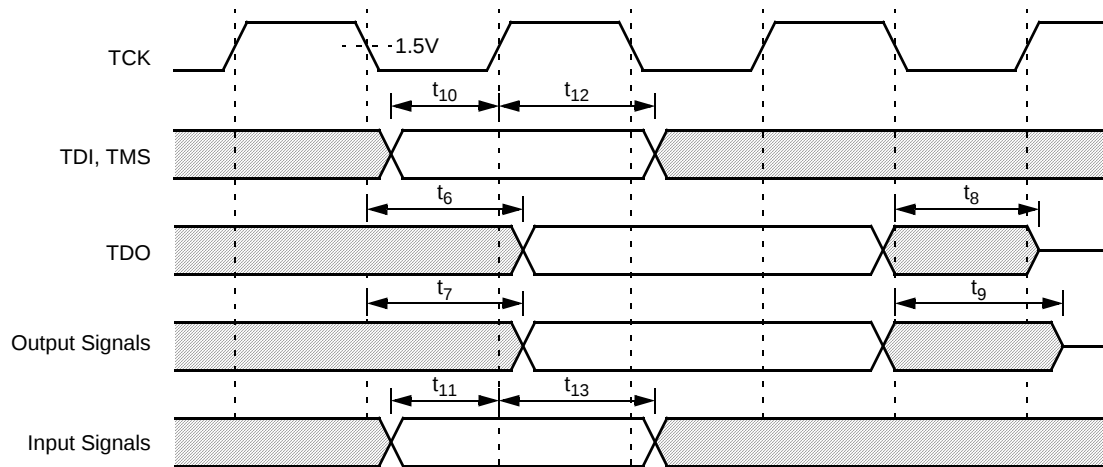
Figure 7-15. JTAG Test Timings
