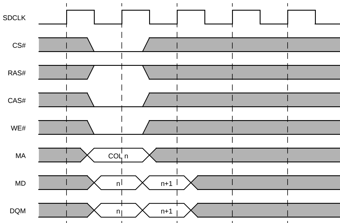
Figure 5-6. Basic Write Cycle
