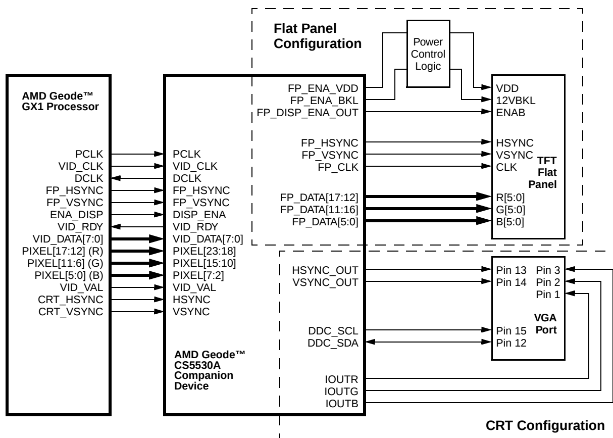
Figure 5-16. Display Controller Signal Connections
