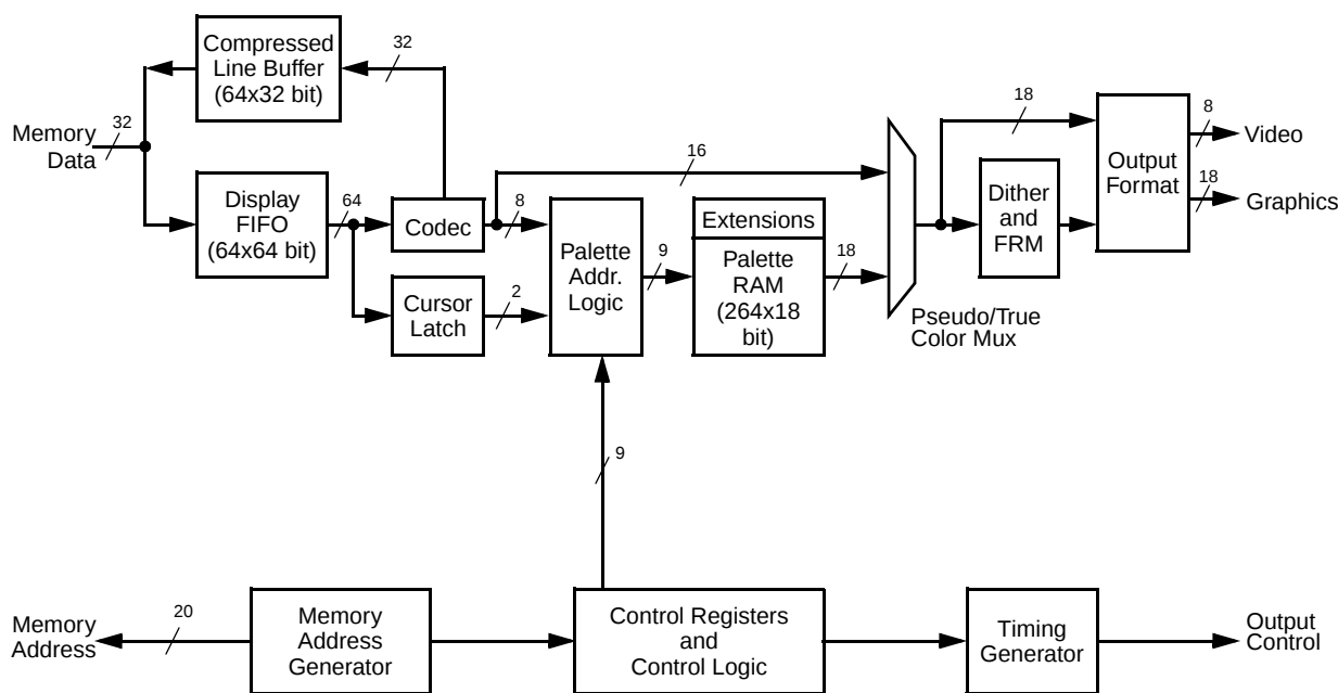
Figure 5-14. Display Controller Block Diagram
