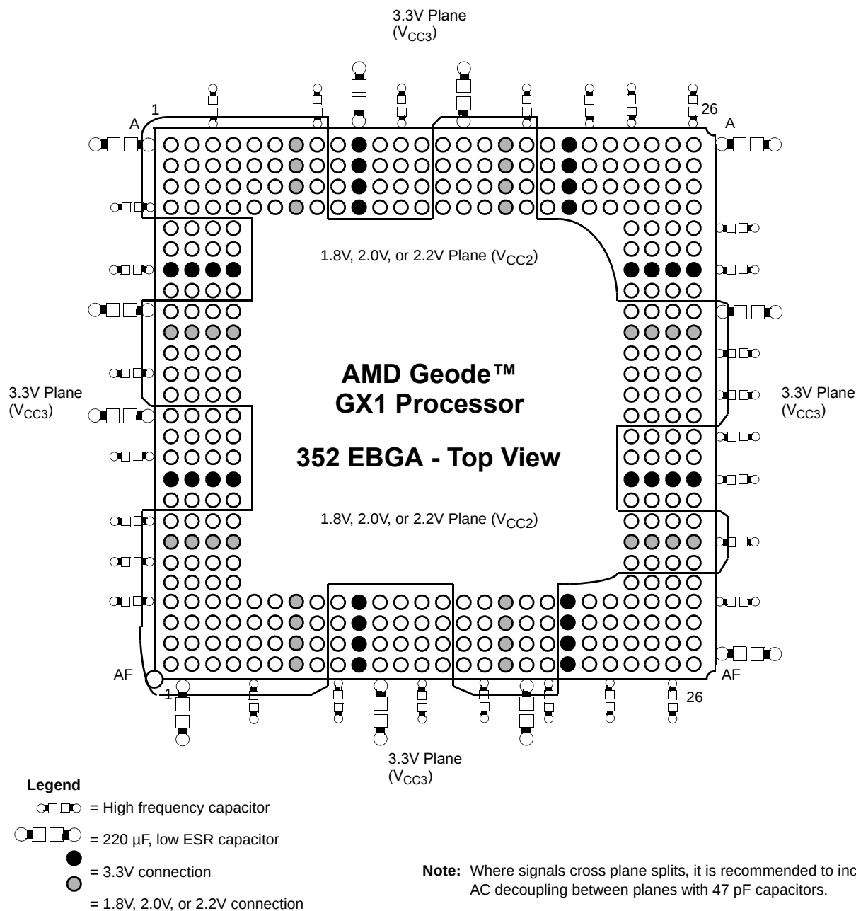
Figure 7-1. EBGA Recommended Split Power Plane and Decoupling
