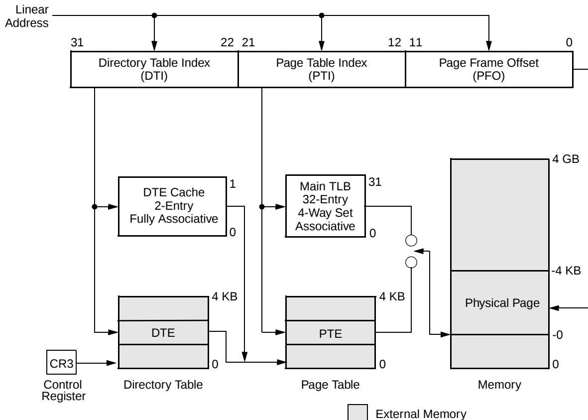
Figure 4-8. Paging Mechanism
