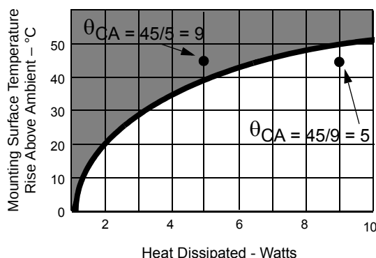
Figure 9-1. Heatsink Example
