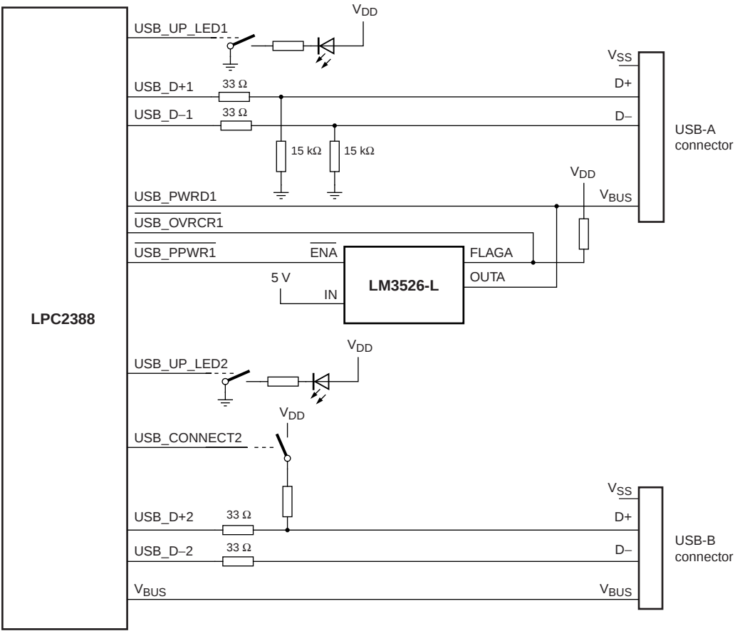
Fig 23. LPC2388 USB OTG port configuration: USB port 2 device, USB port 1 host
