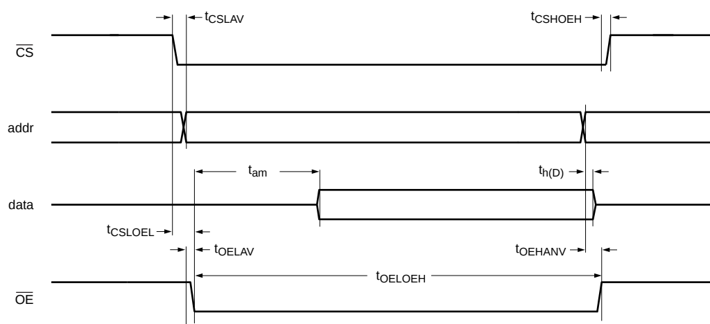
Fig 13. External memory read access
