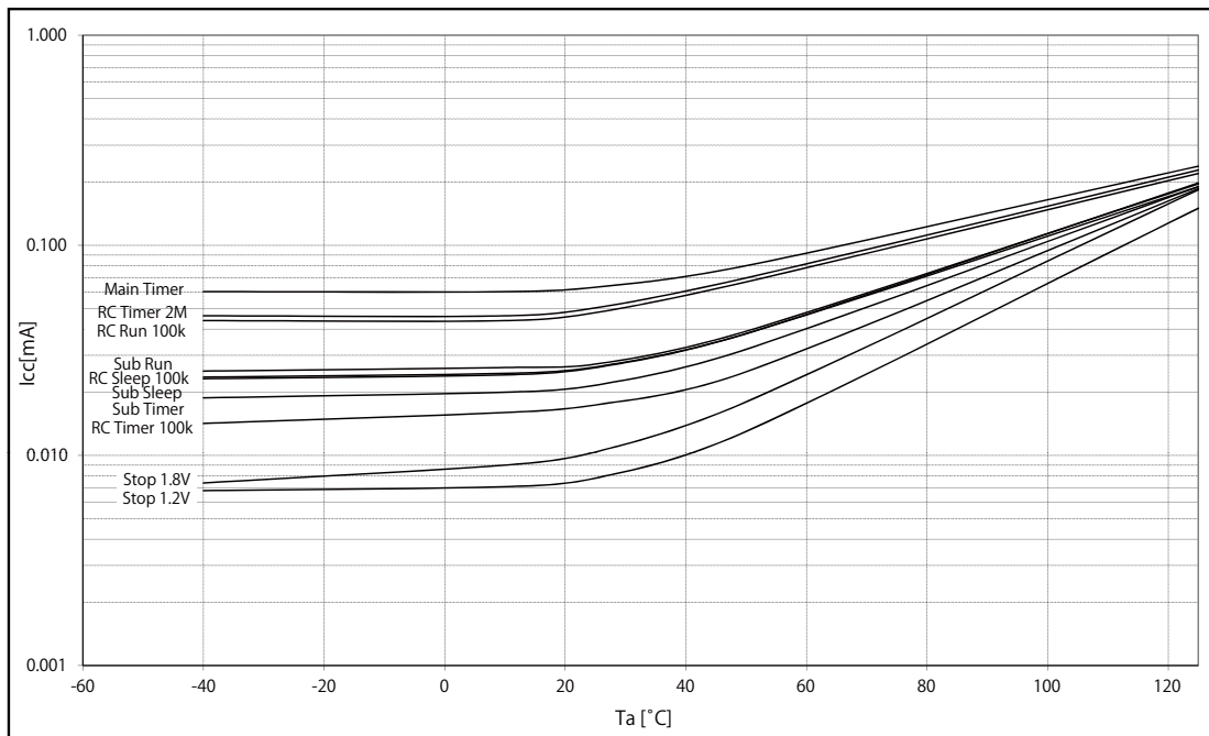
CY96395 Low Power Mode Currents
