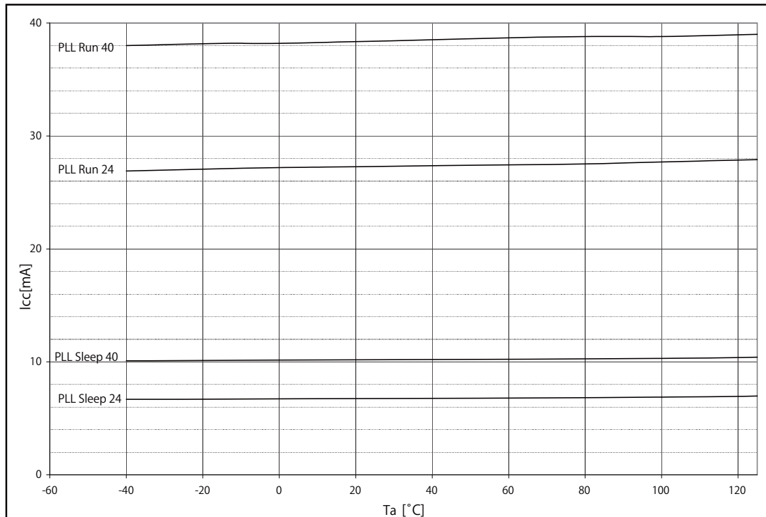
CY96F395 PLL Run and Sleep Mode Currents
