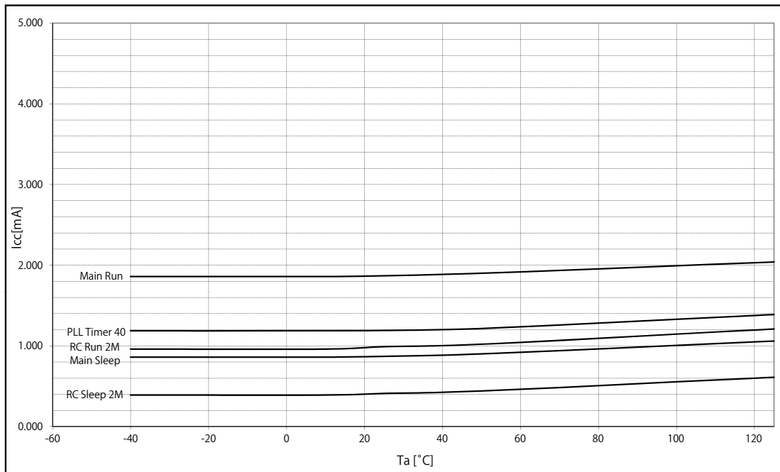
CY96395 Operation Modes with Medium Currents
