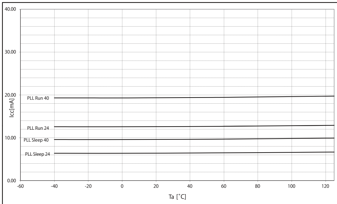
CY96395 PLL Run and Sleep Mode Currents
