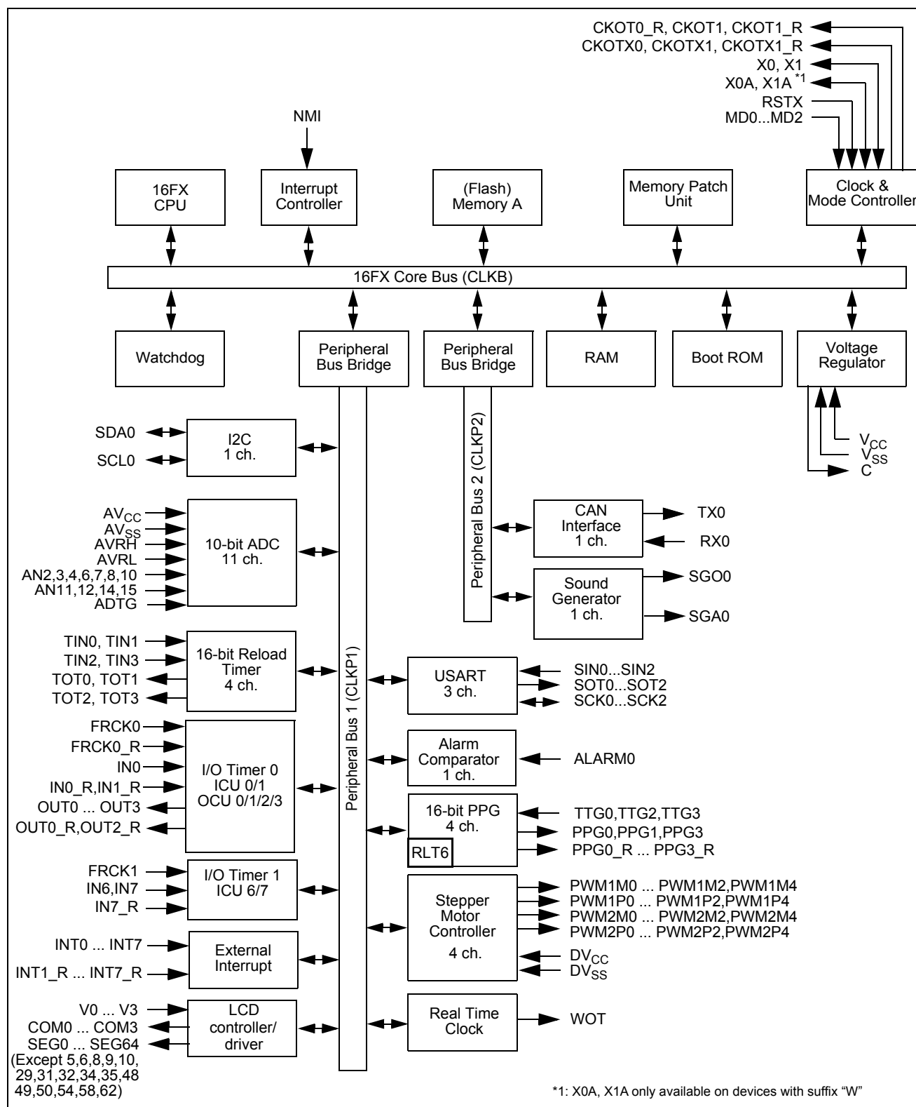
Block Diagram of CY96(F)39x
