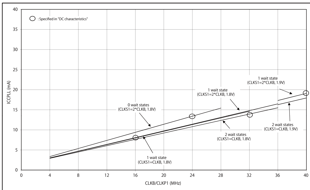
CY96395 PLL Run Mode Current
