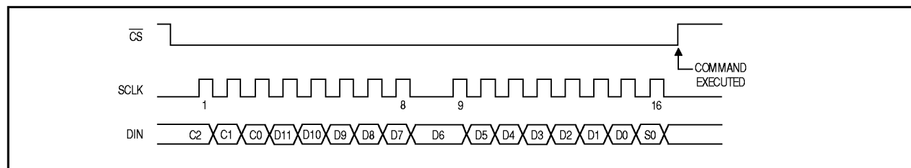
Figure 6. Serial-Interface Timing
