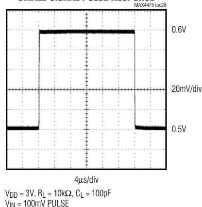
MAX4475-MAX4478 SMALL-SIGNAL PULSE RESPONSE
