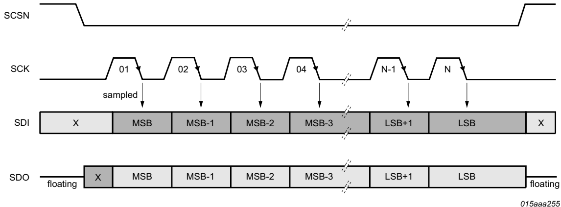
Fig 8. SPI timing protocol
