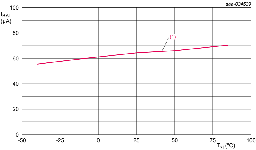
Fig 10. UJA1164A typical Standby quiescent current (μA)
