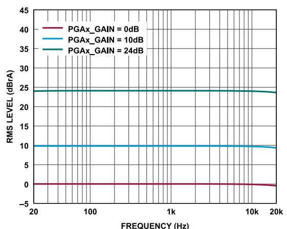
Figure 11. Frequency Response, f_s = 48 kHz, Signal Path = AINxx to SDATAO_x, Differential Mode, Output Relative to PGA Gain Settings (0 dB, 10 dB, and 24 dB), ADCx_FCOMP Off
