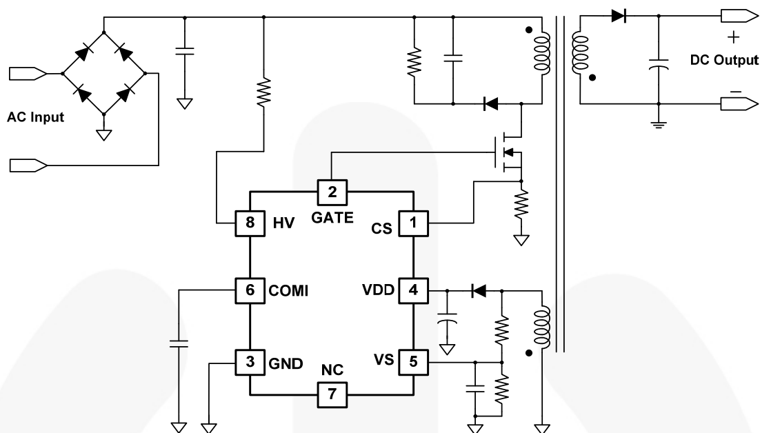
Figure 1. Typical Application
