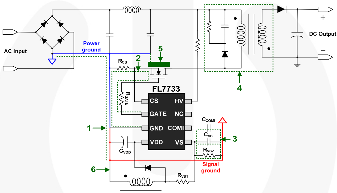
Figure 27. Layout Example
