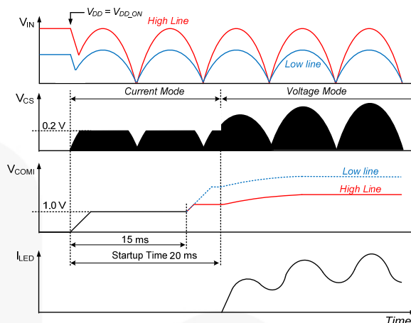
Figure 18. Startup Sequence
