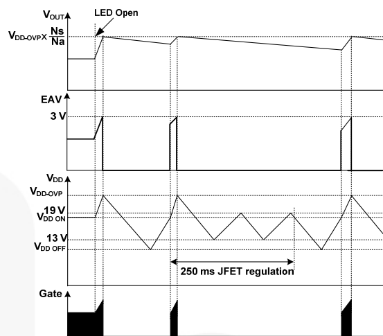
Figure 26. Waveforms in LED Open Condition
