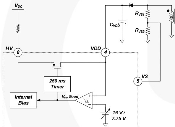
Figure 17. Startup Block
