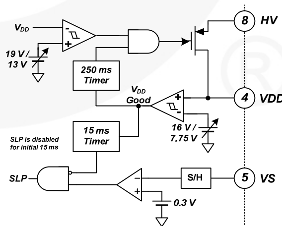
Figure 23. Internal SLP Block
