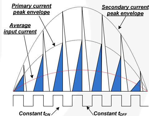
Figure 19. Power Factor Correction
