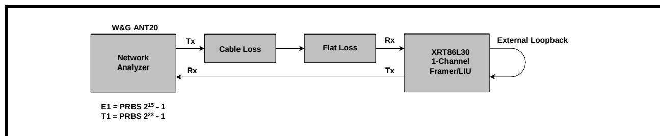
FIGURE 61. TEST CONFIGURATION FOR MEASURING RECEIVE SENSITIVITY
