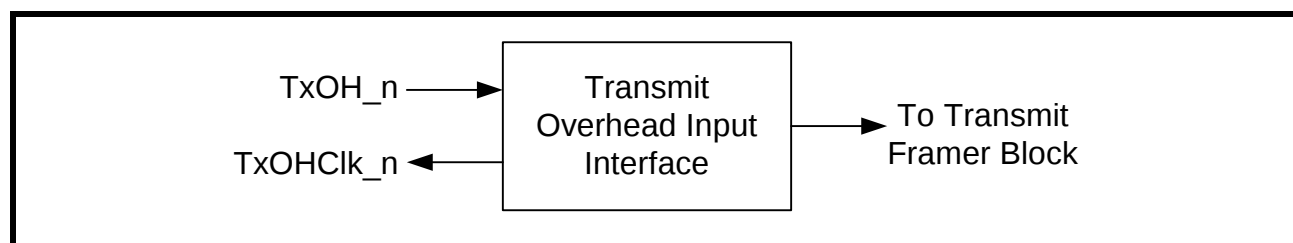
FIGURE 44. BLOCK DIAGRAM OF THE E1 TRANSMIT OVERHEAD INPUT INTERFACE OF XRT86L30
