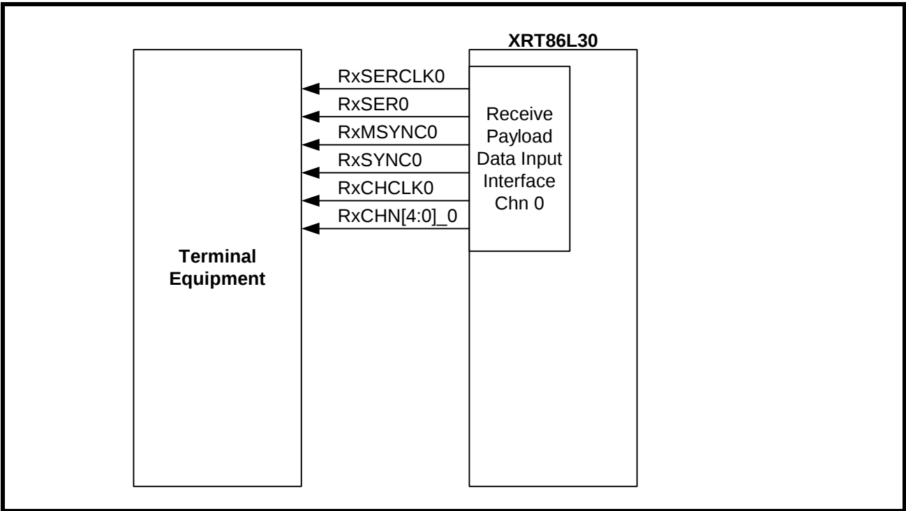
FIGURE 65. INTERFACING THE RECEIVE PATH TO LOCAL TERMINAL EQUIPMENT
