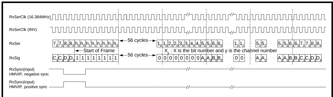
FIGURE 75. WAVEFORMS FOR CONNECTING THE RECEIVE MULTIPLEXED HIGH-SPEED INPUT INTERFACE AT HMVIP 16.384MBIT/S MODE
