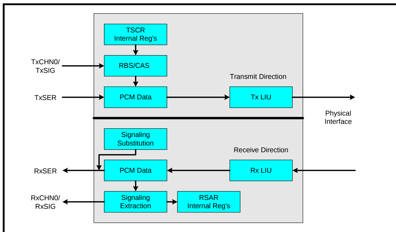
FIGURE 17. ESF / CAS EXTERNAL SIGNALING BUS
