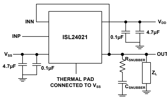
FIGURE 25. OUTPUT SNUBBER CIRCUIT
