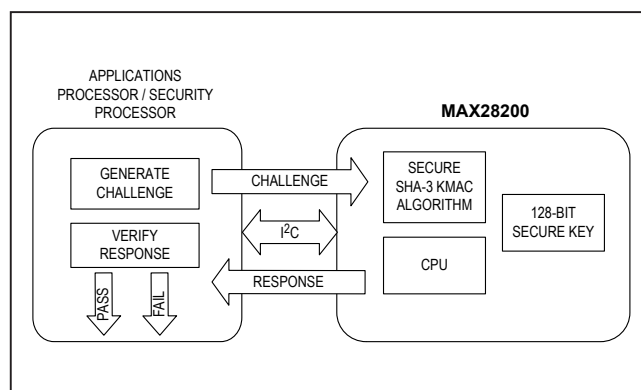
Figure 2. SHA-3 Authentication
