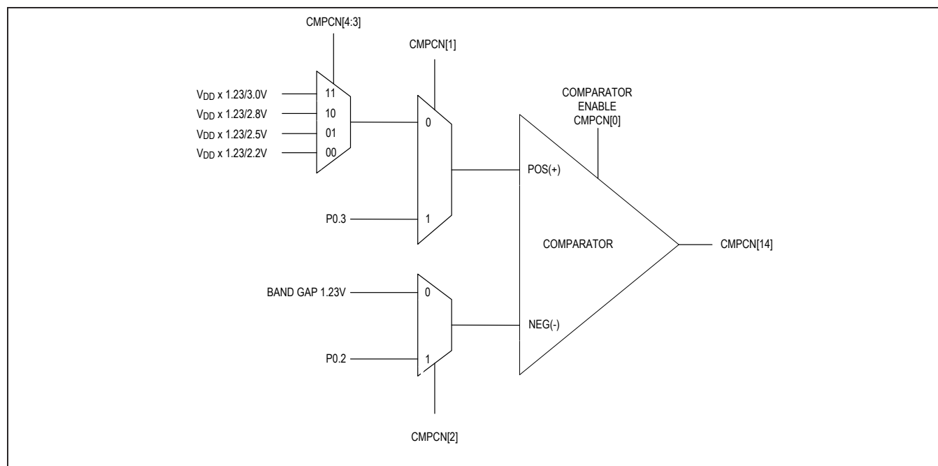
Figure 3. Comparator Configuration
