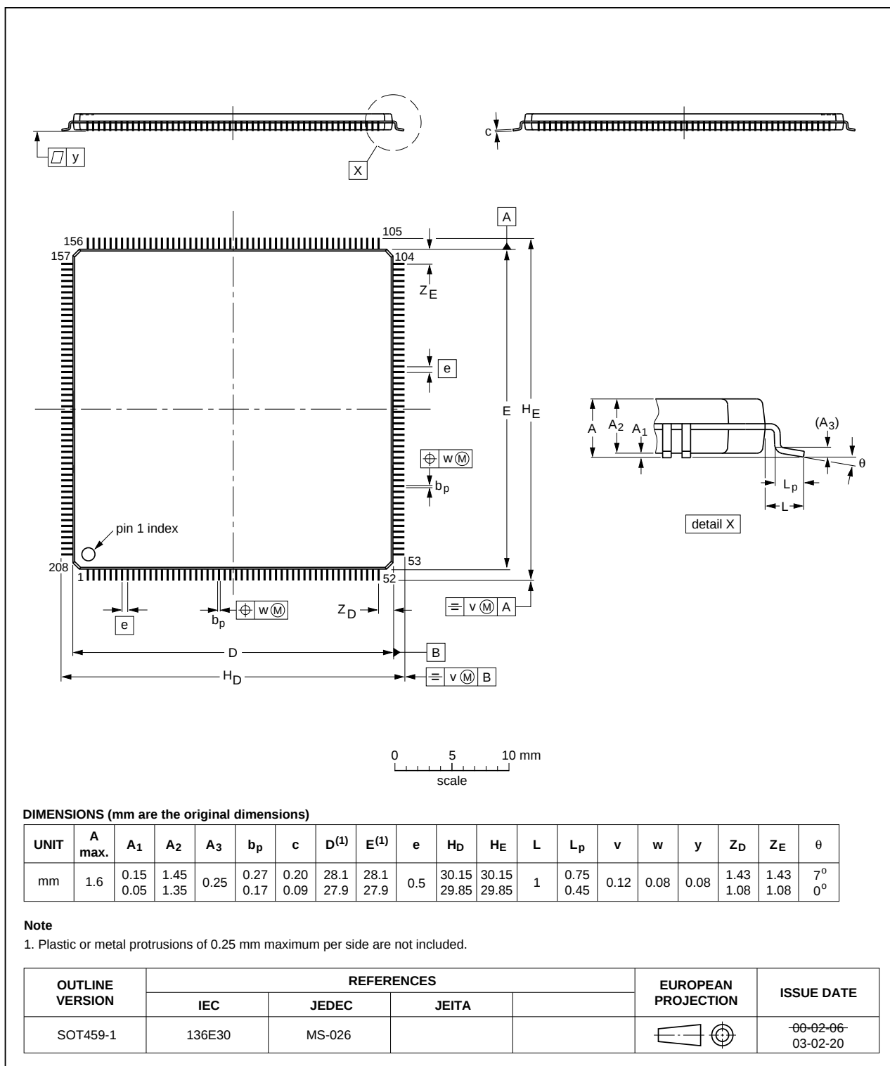
Fig 47. Package outline of the LQFP208 package
