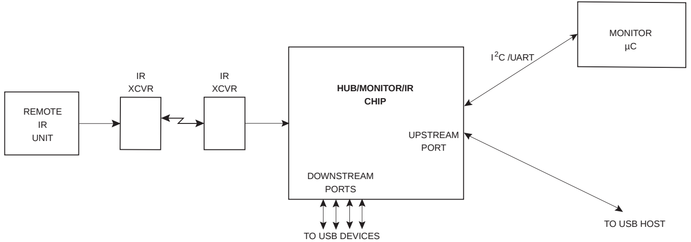
Figure 1. Application Example
