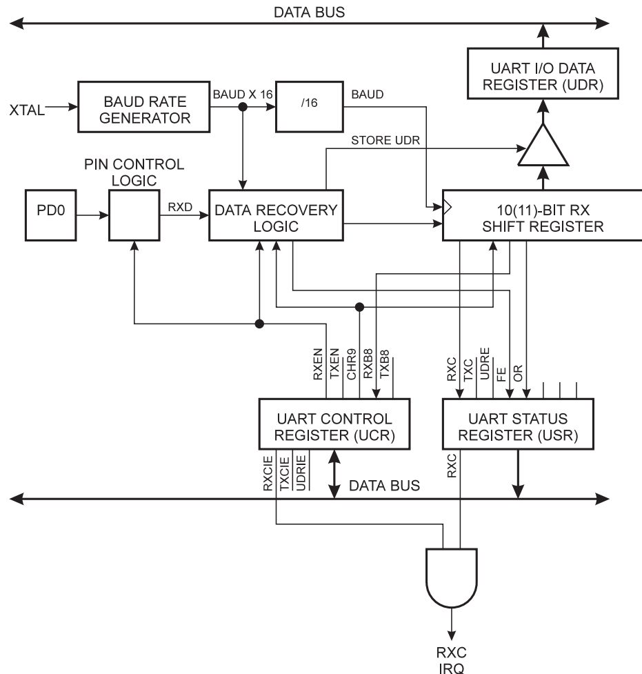
Figure 20. UART Receiver
