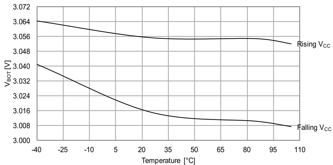
Figure 37-53. BOD Thresholds vs. Temperature BOD level = 3.0V.
