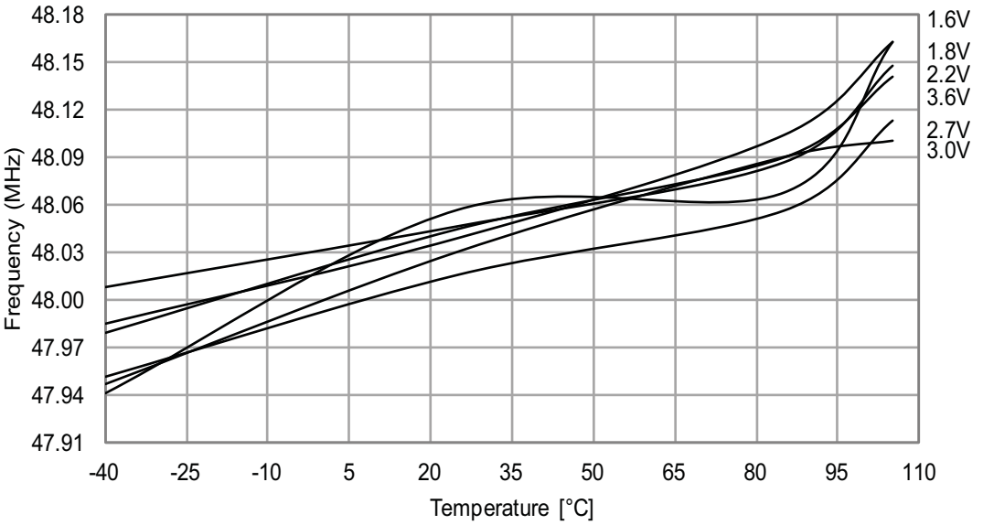
Figure 37-77. 48MHz Internal Oscillator Frequency vs. Temperature DPLL enabled, from the 32.768kHz internal oscillator.
