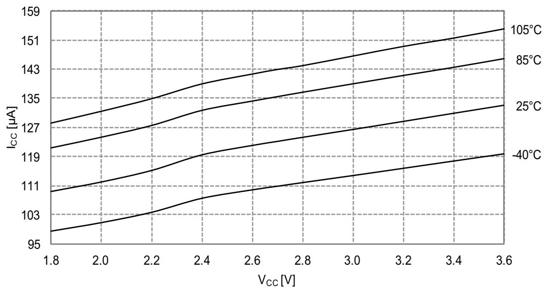
Figure 37-54. BOD Current Consumption vs. V_{CC} Continuous mode, BOD level = 1.6V.
