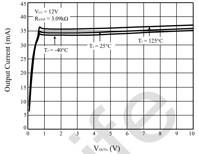
Figure 23 Output Current vs. V_{OUTx} (for Different T_J )
