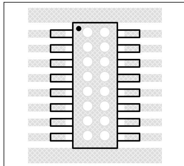
Figure 30 Board Via Layout For Thermal Dissipation
