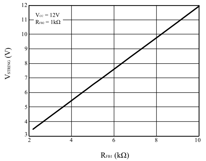
Figure 27 V_{STRING} vs. R_{FB1}
