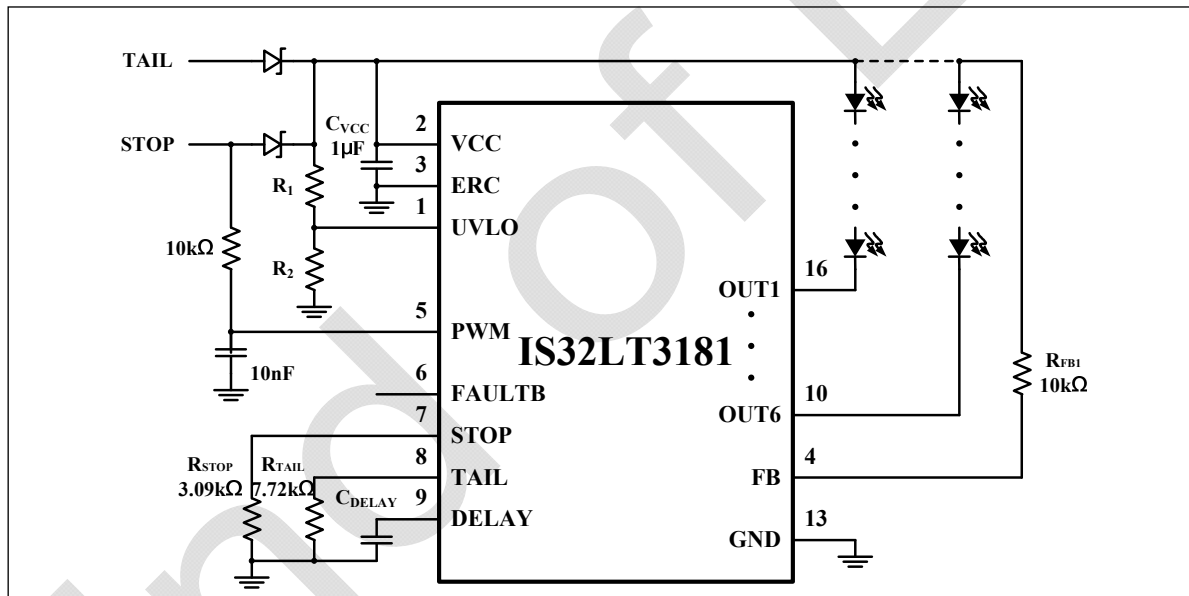
Figure 2 Typical Application Circuit (Without External FET)
