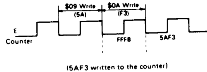
Figure 18 Counter Write Timing
