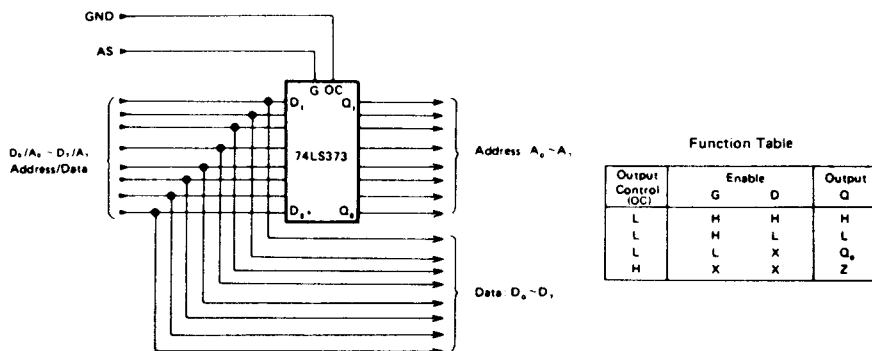
Figure 15 Latch Connection
