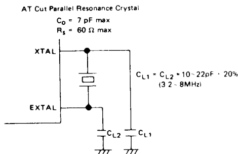
Figure 10 Crystal Interface
