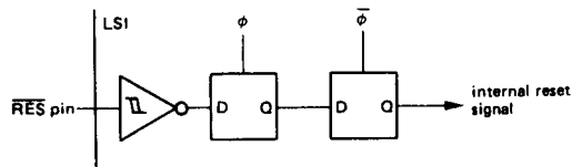
Figure 34 \overline{RES} circuit
