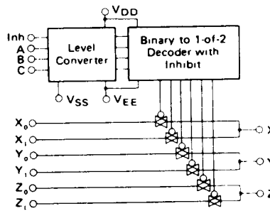
Figure 12 HD14053B Multiplexers/De-Multiplexers
