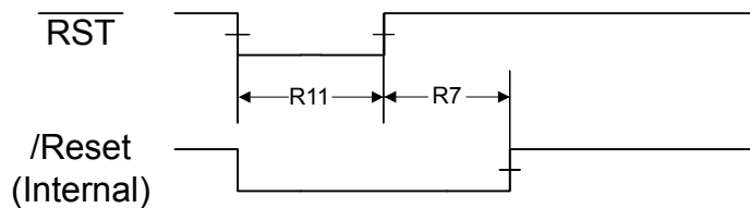
Figure 23-5. External Reset Timing (RST)
