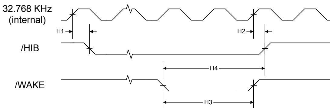
Figure 23-10. Hibernation Module Timing
