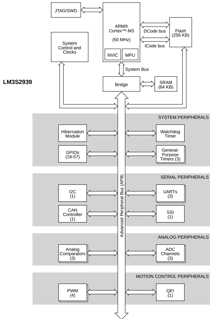
Figure 1-1. Stellaris® LM3S2939 Microcontroller High-Level Block Diagram
