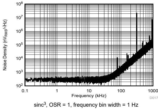
Figure 6-24. Noise Density With Both Inputs Shorted to HGND
