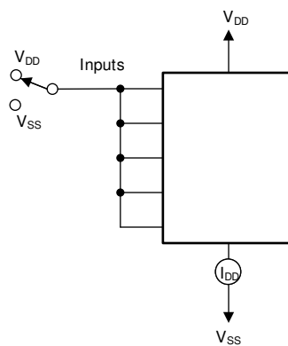
Figure 7-3. Quiescent Device Current Test Circuit
