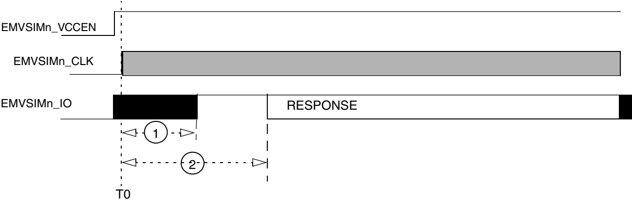
Figure 15. Internal Reset Card Reset Sequence
