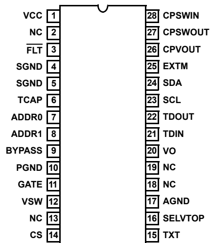
ISL6423B (28 LD EPTSSOP) TOP VIEW
