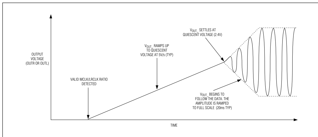
Figure 11. Power-Up Sequence
