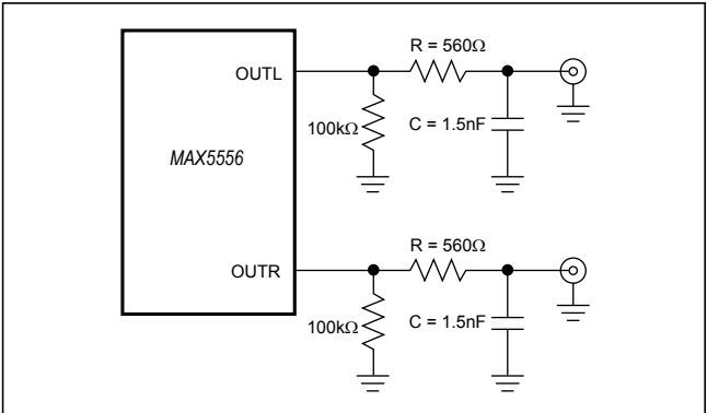
Figure 8. Passive Component Analog Output Filter
