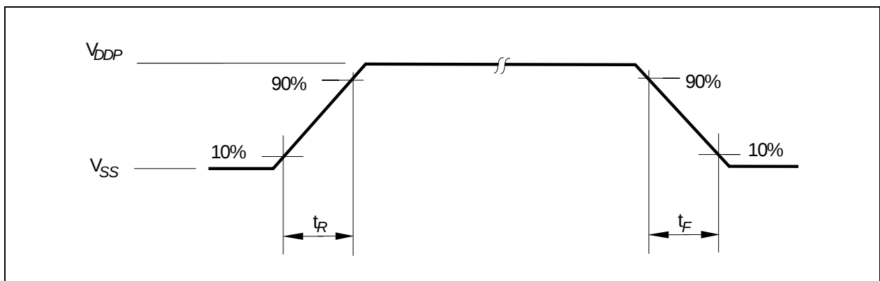
Figure 42 Rise/Fall Times Parameters
