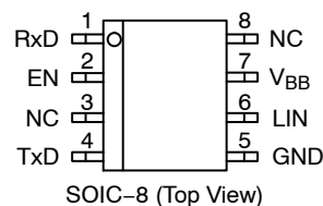
SOIC-8 (Top View)
