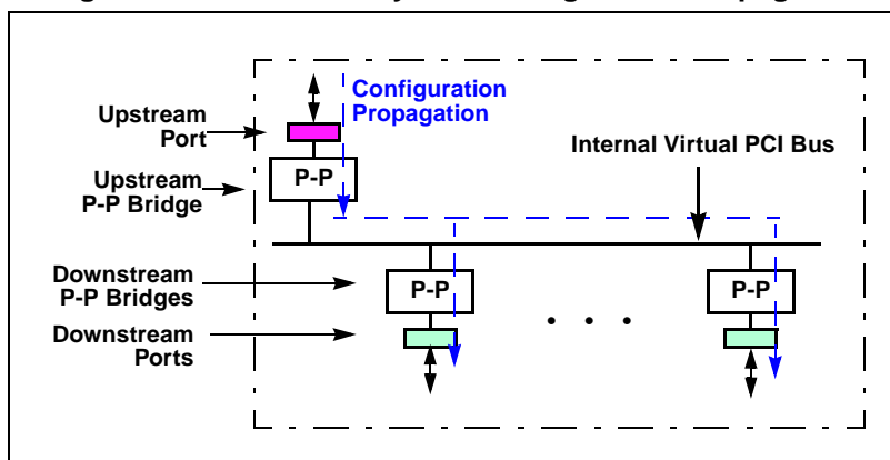
Figure 4-5. PEX 8619 System Configuration Propagation
