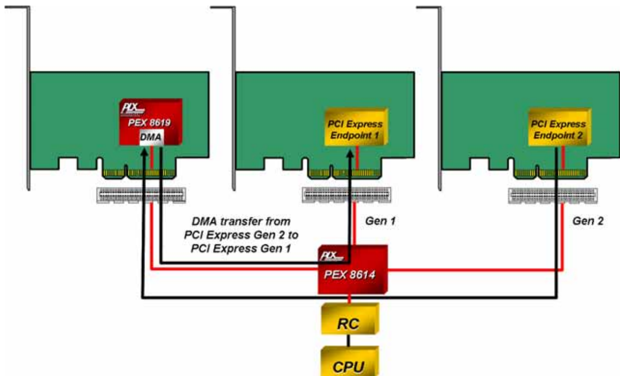
Figure 2-7. Generic Data Mover
