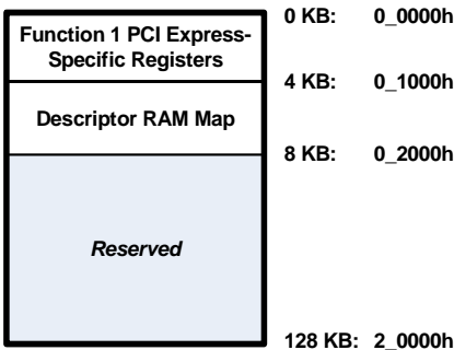
Figure 18-1. DMA BAR0/1 Window
